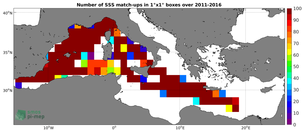
Figure 4: Number of SSS match-ups between TSG (LEGOS-DM) SSS and the SMOS SSS L3 MED-ATL-OA v2 - 9 Days (BEC) SSS product for the Mediterranean Sea Pi-MEP region over 1^\circ \times 1^\circ boxes and for the full satellite product period.
