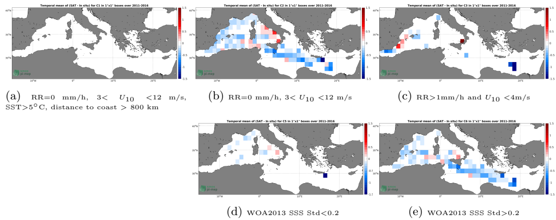
Figure 12: Temporal mean gridded over spatial boxes of size 1^\circ \times 1^\circ of \Delta SSS (SMOS SSS L3 MED-ATL-OA v2 - 9 Days (BEC) - TSG (LEGOS-DM)) for 5 different subdatasets corresponding to:RR=0 mm/h, 3 < U_{10} < 12 m/s, SST >5^\circ C, distance to coast > 800 km (a), RR=0 mm/h, 3 < U_{10} < 12 m/s (b), RR >1 mm/h and U_{10} < 4 m/s (c), WOA2013 SSS Std <0.2 (d), WOA2013 SSS Std >0.2 (e).
