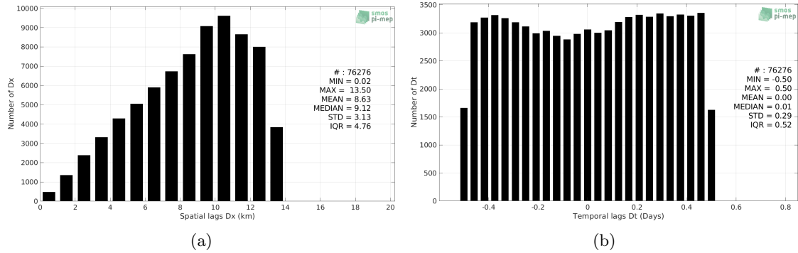
Figure 5: Histograms of the spatial (a) and temporal (b) lags between the location/time of the TSG (LEGOS-DM) measurement and the date of the corresponding SMOS SSS L3 MED-ATL-OA v2 - 9 Days (BEC) SSS pixel.
