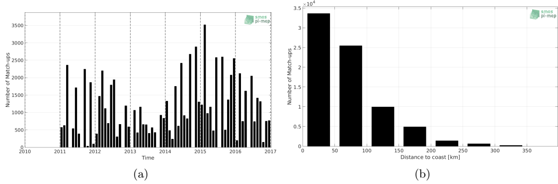
Figure 1: Number of match-ups between TSG-LEGOS-DM and SMOS-L3-BEC-MED-ATL-OA-V2-9DAYS-0.25DEG SSS as a function of time (a) and as function of the distance to coast (b) over the Mediterranean Sea Pi-MEP region and for the full satellite product period.
