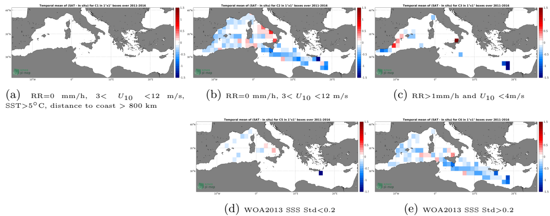
Figure 12: Temporal mean gridded over spatial boxes of size 1^\circ \times 1^\circ of \Delta SSS (SMOS-L3-BEC-MED-ATL-OA-V2-9DAYS-0.25DEG - TSG-LEGOS-DM) for 5 different subdatasets corresponding to:RR=0 mm/h, 3 < U_{10} < 12 m/s, SST >5^\circ\text{C} , distance to coast > 800 km (a), RR=0 mm/h, 3 < U_{10} < 12 m/s (b), RR >1 mm/h and U_{10} < 4 m/s (c), WOA2013 SSS Std <0.2 (d), WOA2013 SSS Std >0.2 (e).
