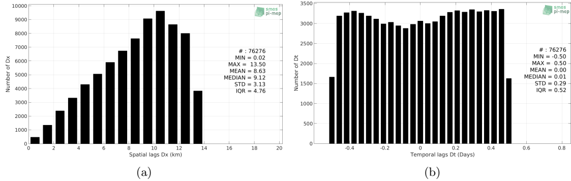
Figure 5: Histograms of the spatial (a) and temporal (b) lags between the time of the TSG-LEGOS-DM measurements and the date of the corresponding SMOS-L3-BEC-MED-ATL-OA-V2-9DAYS-0.25DEG SSS product.
