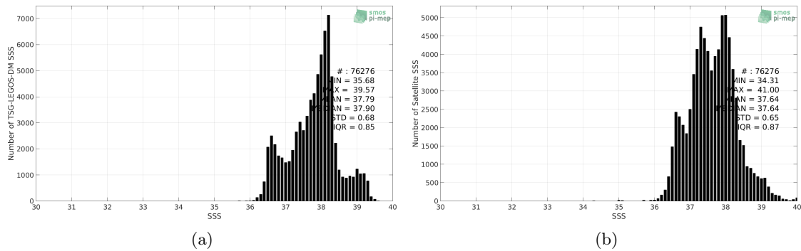
Figure 2: Histograms of SSS from TSG-LEGOS-DM (a) and SMOS-L3-BEC-MED-ATL-OA-V2-9DAYS-0.25DEG (b) considering all match-up pairs per bins of 0.1 over the Mediterranean Sea Pi-MEP region and for the full satellite product period.
