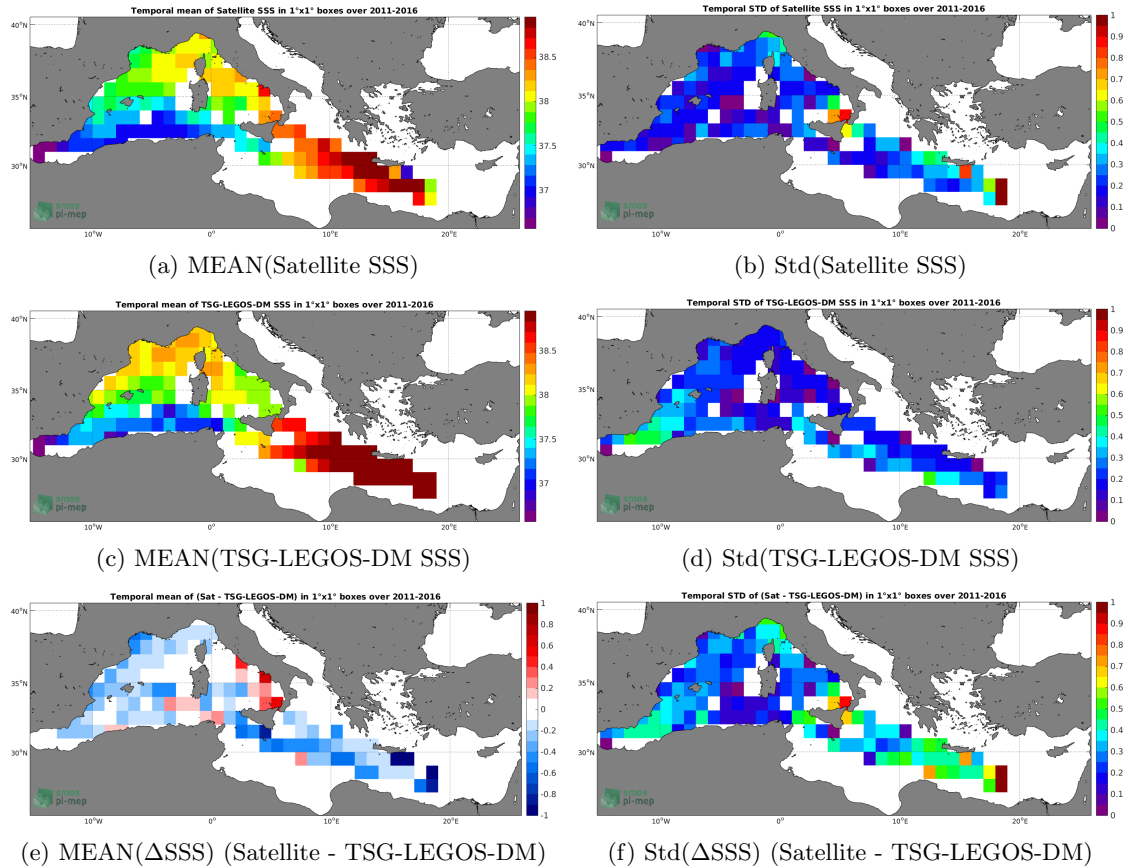
Figure 6: Temporal mean (left) and Std (right) of SSS from SMOS-L3-BEC-MED-ATL-OA-V2-9DAYS-0.25DEG (top), TSG-LEGOS-DM (middle), and of \Delta SSS (Satellite - TSG-LEGOS-DM). Only match-up pairs are used to generate these maps.
