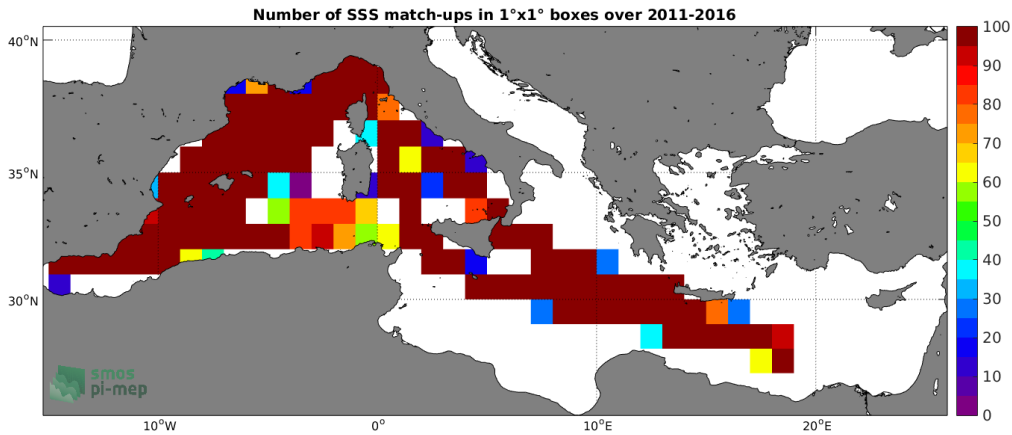
Figure 4: Number of SSS match-ups between TSG-LEGOS-DM SSS and the SMOS-L3-BEC-MED-ATL-OA-V2-9DAYS-0.25DEG SSS product for the Mediterranean Sea Pi-MEP region over 1°x1° boxes and for the full satellite product period.
