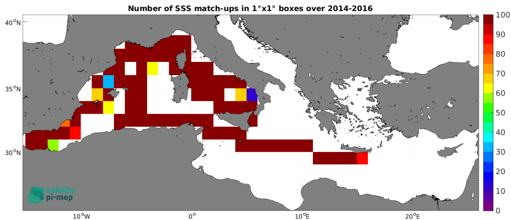
Figure 5: Number of SSS match-ups between TSG (GOSUD-Sailing-ship) SSS and the SMOS SSS L3 MED-ATL-OA v2 - 9 Days (BEC) SSS product for the Mediterranean Sea Pi-MEP region over 1^\circ \times 1^\circ boxes and for the full satellite product period.
