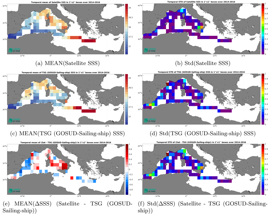
Figure 7: Temporal mean (left) and Std (right) of SSS from SMOS SSS L3 MED-ATL-OA v2 - 9 Days (BEC) (top), TSG (GOSUD-Sailing-ship) (middle), and of \Delta\text{SSS} (Satellite - TSG (GOSUD-Sailing-ship)). Only match-up pairs are used to generate these maps.
