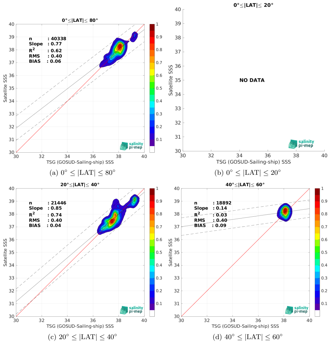
Figure 10: Contour maps of the concentration of SMOS SSS L3 MED-ATL-OA v2 - 9 Days (BEC) SSS (y-axis) versus TSG (GOSUD-Sailing-ship) SSS (x-axis) at match-up pairs for different latitude bands. For each plot, the red line shows x=y . The black thin and dashed lines indicate a linear fit through the data cloud and the \pm 95\% confidence levels, respectively. The number match-up pairs n , the slope and R^2 coefficient of the linear fit, the root mean square (RMS) and the mean bias between satellite and in situ data are indicated for each latitude band in each plots.
