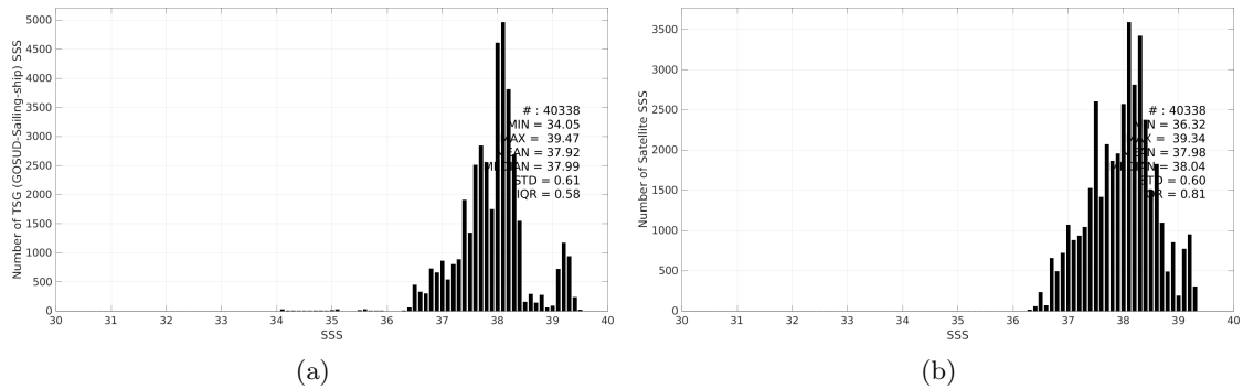
Figure 3: Histograms of SSS from TSG (GOSUD-Sailing-ship) (a) and SMOS SSS L3 MED-ATL-OA v2 - 9 Days (BEC) (b) considering all match-up pairs per bins of 0.1 over the Mediterranean Sea Pi-MEP region and for the full satellite product period.
