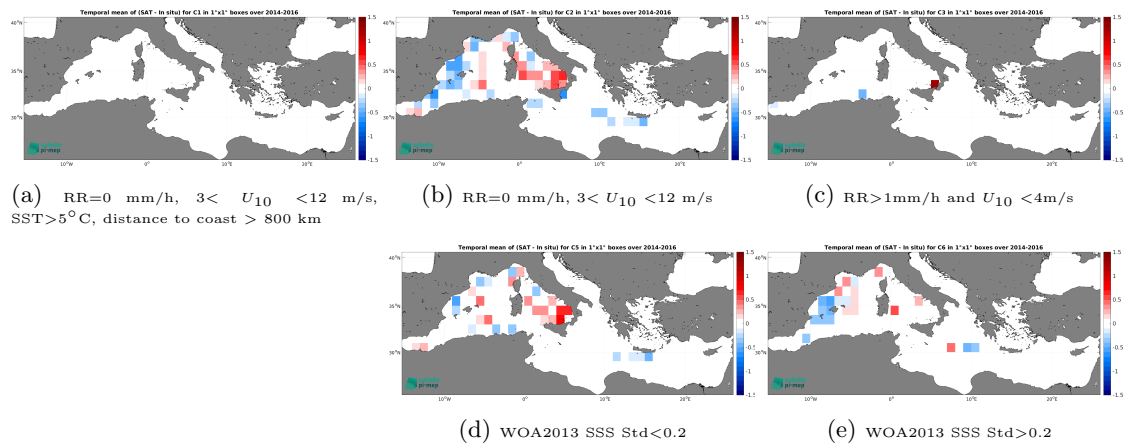
Figure 14: Temporal mean gridded over spatial boxes of size 1^\circ \times 1^\circ of \Delta SSS (SMOS SSS L3 MED-ATL-OA v2 - 9 Days (BEC) - TSG (GOSUD-Sailing-ship)) for 5 different subdatasets corresponding to:RR=0 mm/h, 3 < U_{10} < 12 m/s, SST>5°C, distance to coast > 800 km (a), RR=0 mm/h, 3 < U_{10} < 12 m/s (b), RR>1mm/h and U_{10} < 4 m/s (c), WOA2013 SSS Std<0.2 (d), WOA2013 SSS Std>0.2 (e).
