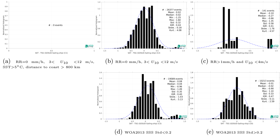
Figure 15: Normalized histogram of \Delta SSS (SMOS SSS L3 MED-ATL-OA v2 - 9 Days (BEC) - TSG (GOSUD-Sailing-ship)) for 5 different subdatasets corresponding to: RR=0 mm/h, 3 < U_{10} < 12 m/s, SST > 5°C, distance to coast > 800 km (a), RR=0 mm/h, 3 < U_{10} < 12 m/s (b), RR > 1mm/h and U_{10} < 4 m/s (c), WOA2013 SSS Std < 0.2 (d), WOA2013 SSS Std > 0.2 (e).
