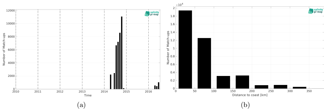
Figure 2: Number of match-ups between TSG (GOSUD-Sailing-ship) and SMOS SSS L3 MED-ATL-OA v2 - 9 Days (BEC) SSS as a function of time (a) and as function of the distance to coast (b) over the Mediterranean Sea Pi-MEP region and for the full satellite product period.
