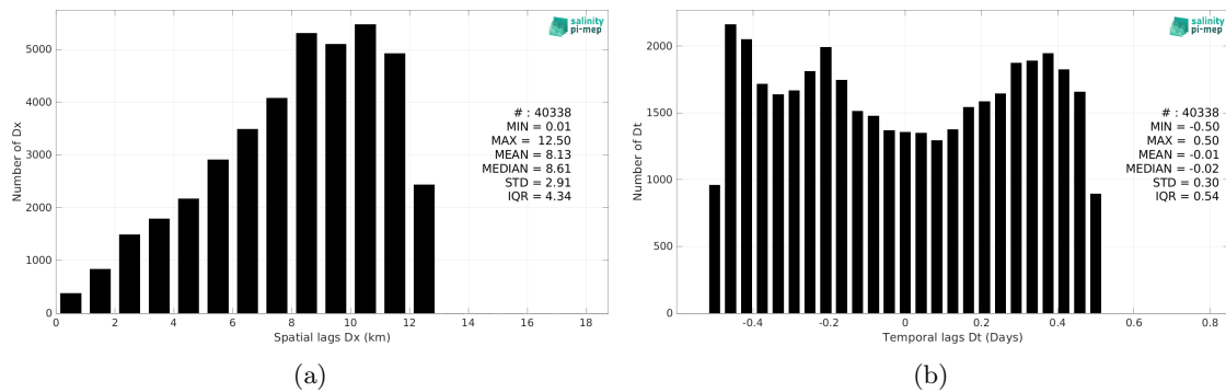
Figure 6: Histograms of the spatial (a) and temporal (b) lags between the location/time of the TSG (GOSUD-Sailing-ship) measurement and the date of the corresponding SMOS SSS L3 MED-ATL-OA v2 - 9 Days (BEC) SSS pixel.
