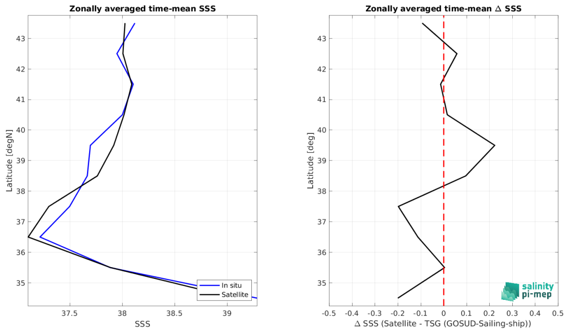
Figure 9: Left panel: Zonal mean SSS from SMOS SSS L3 MED-ATL-OA v2 - 9 Days (BEC) satellite product (black) and from TSG (GOSUD-Sailing-ship) (blue). Right panel: Zonal mean of \Delta SSS (Satellite - TSG (GOSUD-Sailing-ship)) for all the collected Pi-MEP match-up pairs estimated over the full satellite product period.
