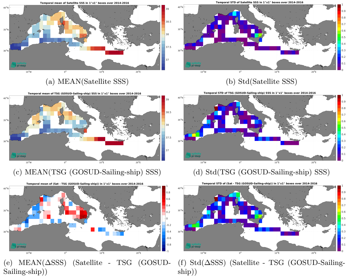
Figure 6: Temporal mean (left) and Std (right) of SSS from SMOS SSS L3 MED-ATL-OA v2 - 9 Days (BEC) (top), TSG (GOSUD-Sailing-ship) (middle), and of \Delta\text{SSS} (Satellite - TSG (GOSUD-Sailing-ship)). Only match-up pairs are used to generate these maps.
