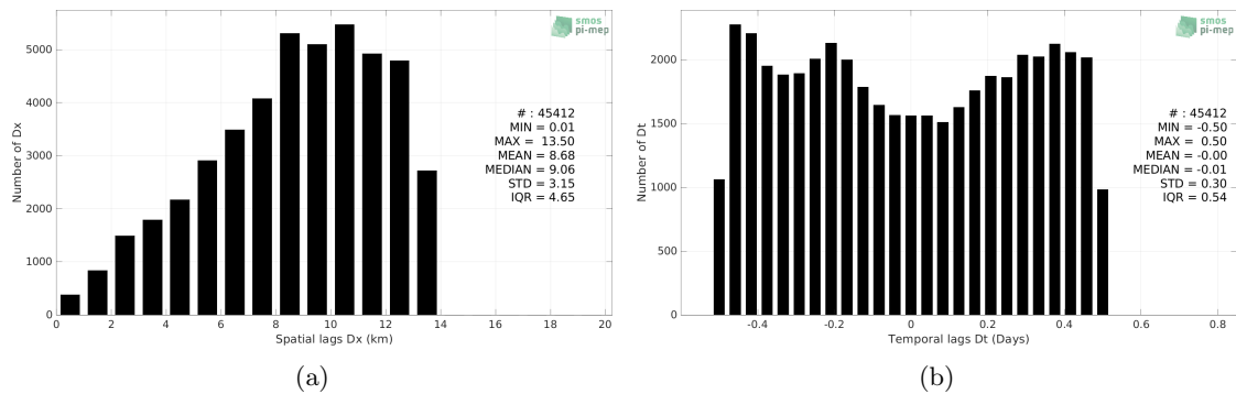
Figure 5: Histograms of the spatial (a) and temporal (b) lags between the location/time of the TSG (GOSUD-Sailing-ship) measurement pixel and the date of the corresponding SMOS SSS L3 MED-ATL-OA v2 - 9 Days (BEC) SSS pixel.
