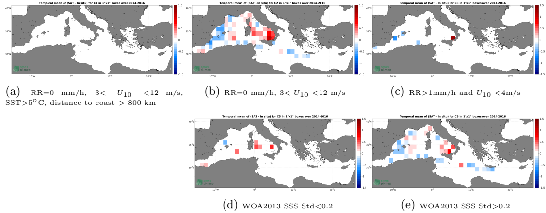
Figure 12: Temporal mean gridded over spatial boxes of size 1^{\circ}\times 1^{\circ} of \Delta SSS (SMOS SSS L3 MED-ATL-OA v2 - 9 Days (BEC) - TSG (GOSUD-Sailing-ship)) for 5 different subdatasets corresponding to:RR=0 mm/h, 3 < U_{10} < 12 m/s, SST >5^{\circ}\text{C} , distance to coast > 800 km (a), RR=0 mm/h, 3 < U_{10} < 12 m/s (b), RR >1 mm/h and U_{10} < 4 m/s (c), WOA2013 SSS Std <0.2 (d), WOA2013 SSS Std >0.2 (e).
