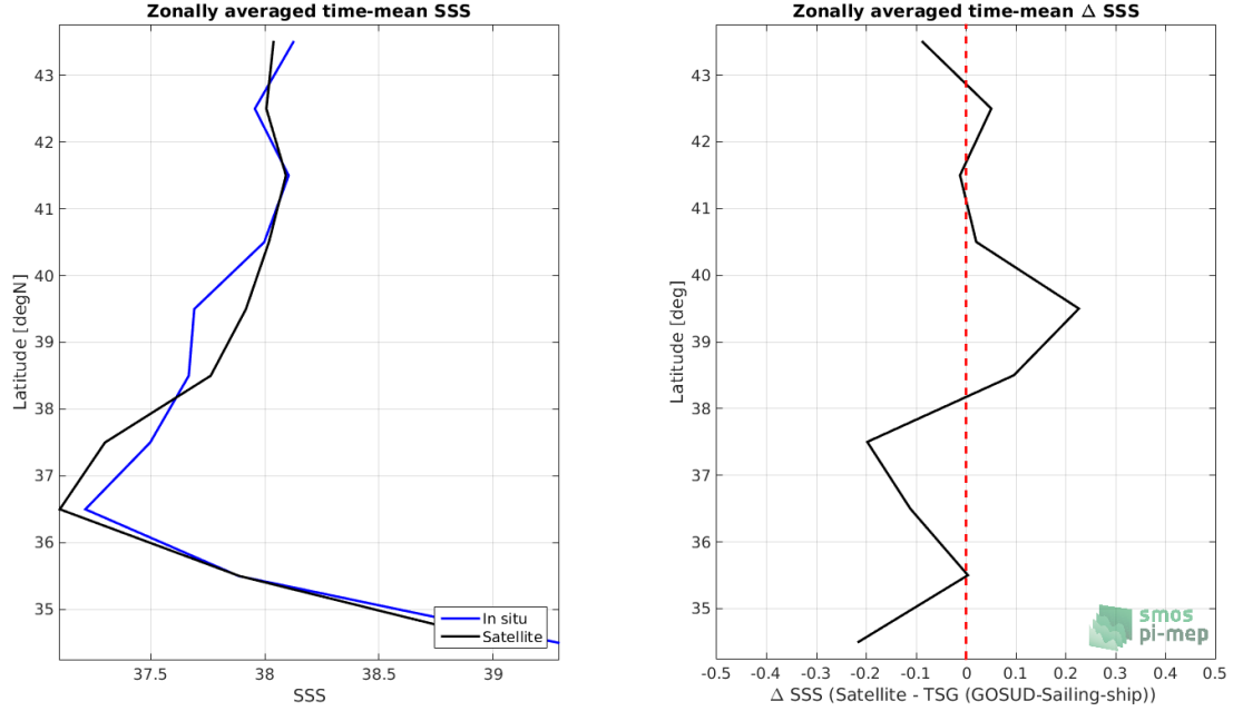
Figure 8: Left panel: Zonal mean SSS from SMOS SSS L3 MED-ATL-OA v2 - 9 Days (BEC) satellite product (black) and from TSG (GOSUD-Sailing-ship) (blue). Right panel: Zonal mean of \Delta SSS (Satellite - TSG (GOSUD-Sailing-ship)) for all the collected Pi-MEP match-up pairs estimated over the full satellite product period.
