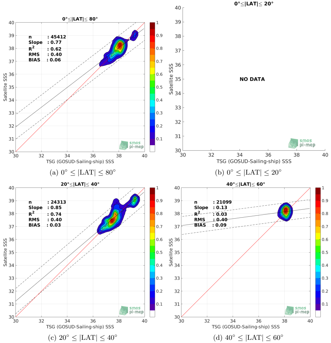
Figure 9: Contour maps of the concentration of SMOS SSS L3 MED-ATL-OA v2 - 9 Days (BEC) SSS (y-axis) versus TSG (GOSUD-Sailing-ship) SSS (x-axis) at match-up pairs for different latitude bands. For each plot, the red line shows x=y . The black thin and dashed lines indicate a linear fit through the data cloud and the \pm 95\% confidence levels, respectively. The number match-up pairs n , the slope and R^2 coefficient of the linear fit, the root mean square (RMS) and the mean bias between satellite and in situ data are indicated for each latitude band in each plots.
