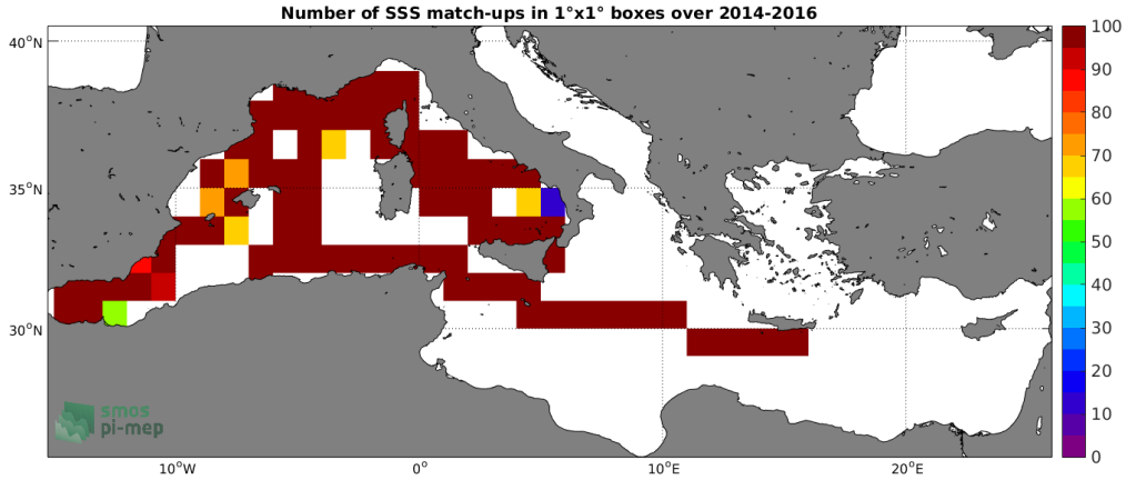
Figure 4: Number of SSS match-ups between TSG (GOSUD-Sailing-ship) SSS and the SMOS SSS L3 MED-ATL-OA v2 - 9 Days (BEC) SSS product for the Mediterranean Sea Pi-MEP region over 1^\circ \times 1^\circ boxes and for the full satellite product period.
