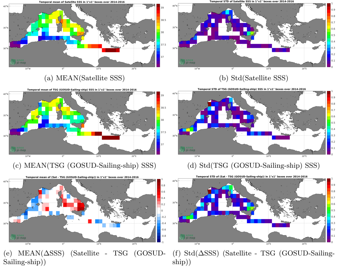
Figure 6: Temporal mean (left) and Std (right) of SSS from SMOS SSS L3 MED-ATL-OA v2 - 9 Days (BEC) (top), TSG (GOSUD-Sailing-ship) (middle), and of \Delta SSS (Satellite - TSG (GOSUD-Sailing-ship)). Only match-up pairs are used to generate these maps.
