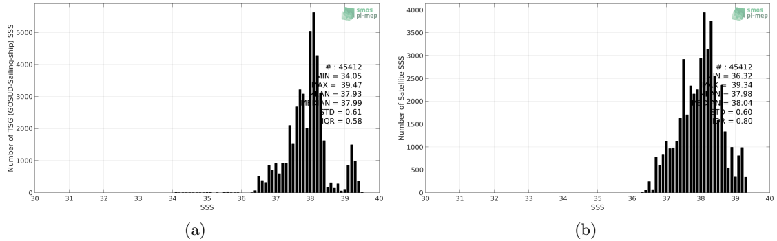
Figure 2: Histograms of SSS from TSG (GOSUD-Sailing-ship) (a) and SMOS SSS L3 MED-ATL-OA v2 - 9 Days (BEC) (b) considering all match-up pairs per bins of 0.1 over the Mediterranean Sea Pi-MEP region and for the full satellite product period.
