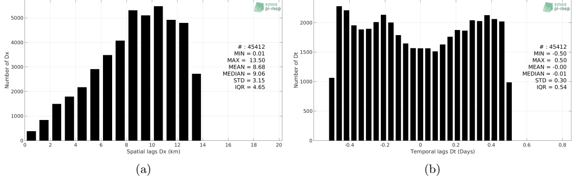
Figure 5: Histograms of the spatial (a) and temporal (b) lags between the location/time of the TSG (GOSUD-Sailing-ship) measurement and the date of the corresponding SMOS SSS L3 MED-ATL-OA v2 - 9 Days (BEC) SSS pixel.
