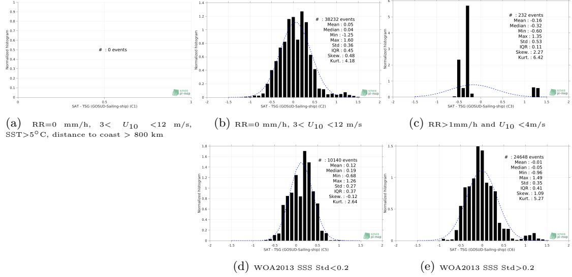
Figure 13: Normalized histogram of \Delta\text{SSS} (SMOS SSS L3 MED-ATL-OA v2 - 9 Days (BEC) - TSG (GOSUD-Sailing-ship)) for 5 different subdatasets corresponding to: RR=0 mm/h, 3 < U_{10} < 12 m/s, SST > 5^\circ\text{C} , distance to coast > 800 km (a), RR=0 mm/h, 3 < U_{10} < 12 m/s (b), RR > 1\text{mm/h} and U_{10} < 4\text{m/s} (c), WOA2013 SSS Std < 0.2 (d), WOA2013 SSS Std > 0.2 (e).
