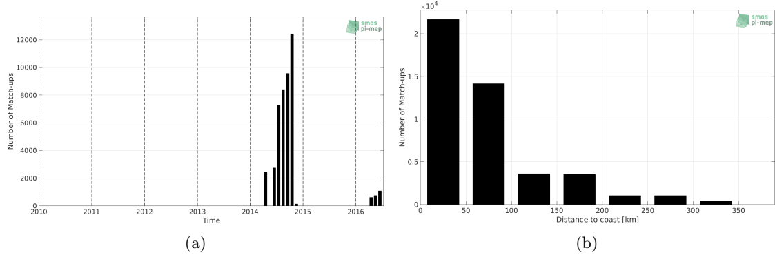
Figure 1: Number of match-ups between TSG (GOSUD-Sailing-ship) and SMOS SSS L3 MED-ATL-OA v2 - 9 Days (BEC) SSS as a function of time (a) and as function of the distance to coast (b) over the Mediterranean Sea Pi-MEP region and for the full satellite product period.
