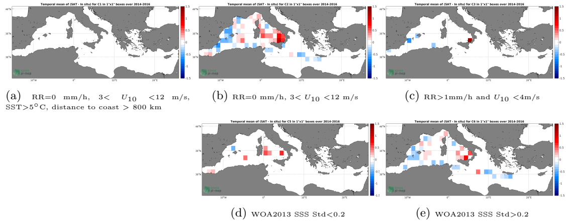
Figure 12: Temporal mean gridded over spatial boxes of size 1^\circ \times 1^\circ of \Delta SSS (SMOS SSS L3 MED-ATL-OA v2 - 9 Days (BEC) - TSG (GOSUD-Sailing-ship)) for 5 different subdatasets corresponding to: RR=0 mm/h, 3 < U_{10} < 12 m/s, SST >5^\circ\text{C} , distance to coast > 800 km (a), RR=0 mm/h, 3 < U_{10} < 12 m/s (b), RR >1 mm/h and U_{10} < 4 m/s (c), WOA2013 SSS Std <0.2 (d), WOA2013 SSS Std >0.2 (e).
