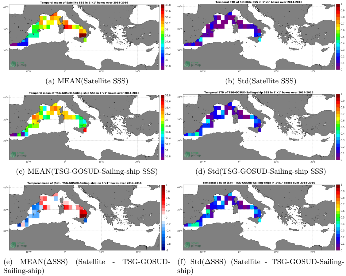
Figure 6: Temporal mean (left) and Std (right) of SSS from SMOS-L3-BEC-MED-ATL-OA-V2-9DAYS-0.25DEG (top), TSG-GOSUD-Sailing-ship (middle), and of \Delta SSS (Satellite - TSG-GOSUD-Sailing-ship). Only match-up pairs are used to generate these maps.
