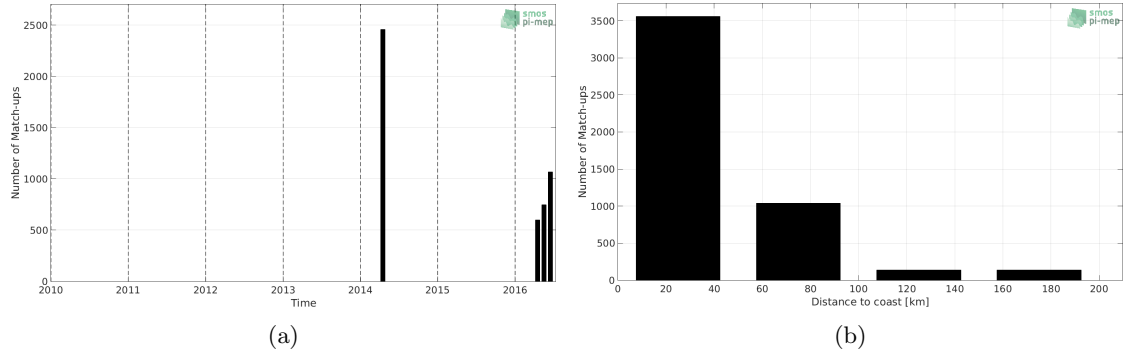
Figure 1: Number of match-ups between TSG-GOSUD-Sailing-ship and SMOS-L3-BEC-MED-ATL-OA-V2-9DAYS-0.25DEG SSS as a function of time (a) and as function of the distance to coast (b) over the Mediterranean Sea Pi-MEP region and for the full satellite product period.
