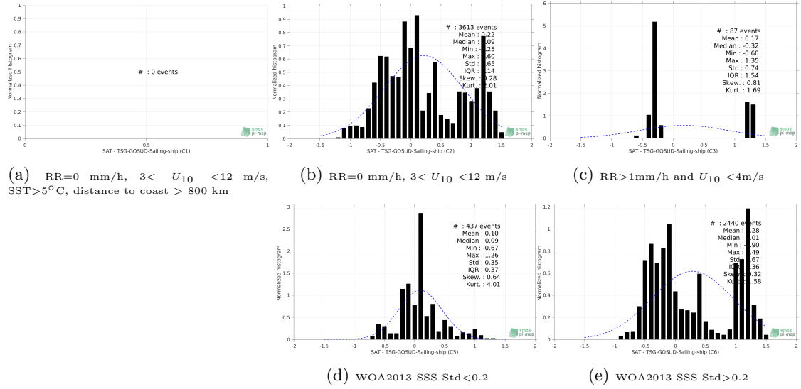
Figure 13: Normalized histogram of \Delta\text{SSS} (SMOS-L3-BEC-MED-ATL-OA-V2-9DAYS-0.25DEG - TSG-GOSUD-Sailing-ship) for 5 different subdatasets corresponding to: RR=0 mm/h, 3 < U_{10} < 12 m/s, SST > 5^\circ\text{C} , distance to coast > 800 km (a), RR=0 mm/h, 3 < U_{10} < 12 m/s (b), RR > 1\text{mm/h} and U_{10} < 4\text{m/s} (c), WOA2013 SSS Std < 0.2 (d), WOA2013 SSS Std > 0.2 (e).
