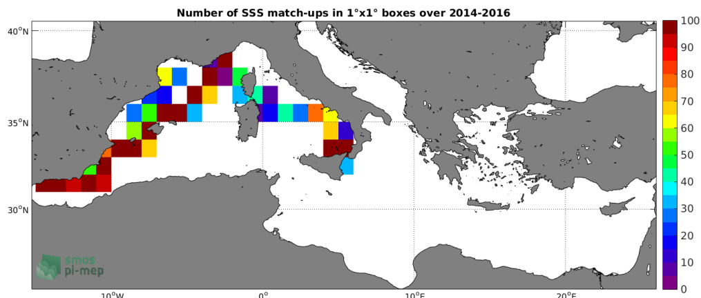
Figure 4: Number of SSS match-ups between TSG-GOSUD-Sailing-ship SSS and the SMOS-L3-BEC-MED-ATL-OA-V2-9DAYS-0.25DEG SSS product for the Mediterranean Sea Pi-MEP region over 1°x1° boxes and for the full satellite product period.
