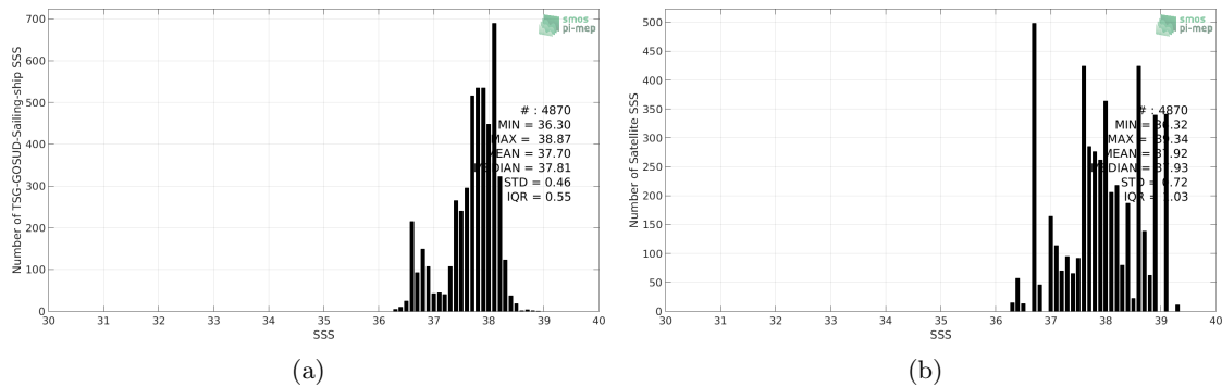
Figure 2: Histograms of SSS from TSG-GOSUD-Sailing-ship (a) and SMOS-L3-BEC-MED-ATL-OA-V2-9DAYS-0.25DEG (b) considering all match-up pairs per bins of 0.1 over the Mediterranean Sea Pi-MEP region and for the full satellite product period.
