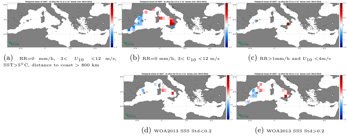
Figure 12: Temporal mean gridded over spatial boxes of size 1^\circ \times 1^\circ of \Delta SSS (SMOS-L3-BEC-MED-ATL-OA-V2-9DAYS-0.25DEG - TSG-GOSUD-Sailing-ship) for 5 different subdatasets corresponding to: RR=0 mm/h, 3 < U_{10} < 12 m/s, SST > 5^\circ C , distance to coast > 800 km (a), RR=0 mm/h, 3 < U_{10} < 12 m/s (b), RR > 1 mm/h and U_{10} < 4 m/s (c), WOA2013 SSS Std < 0.2 (d), WOA2013 SSS Std > 0.2 (e).
