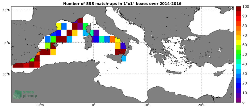
Figure 4: Number of SSS match-ups between TSG-GOSUD-Sailing-ship SSS and the SMOS-L3-BEC-MED-ATL-OA-V2-9DAYS-0.25DEG SSS product for the Mediterranean Sea Pi-MEP region over 1^\circ \times 1^\circ boxes and for the full satellite product period.
