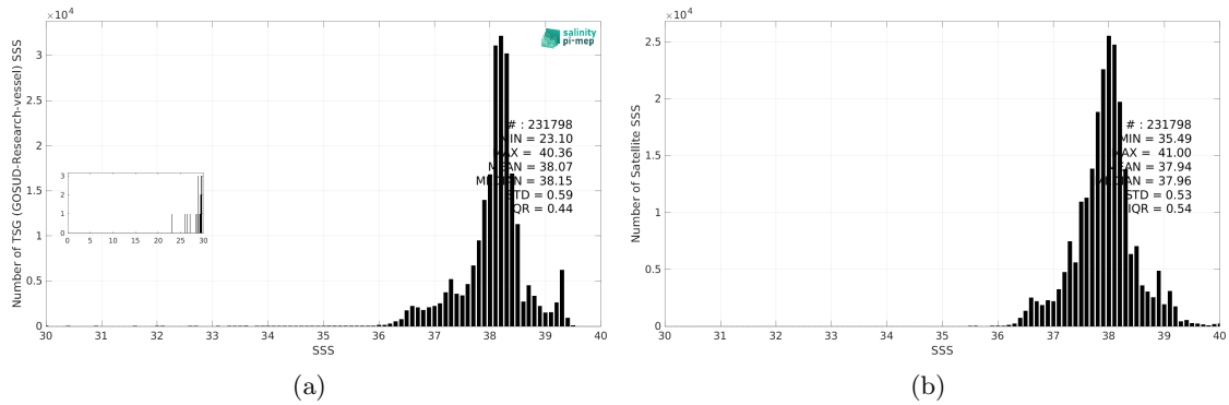
Figure 3: Histograms of SSS from TSG (GOSUD-Research-vessel) (a) and SMOS SSS L3 MED-ATL-OA v2 - 9 Days (BEC) (b) considering all match-up pairs per bins of 0.1 over the Mediterranean Sea Pi-MEP region and for the full satellite product period.
