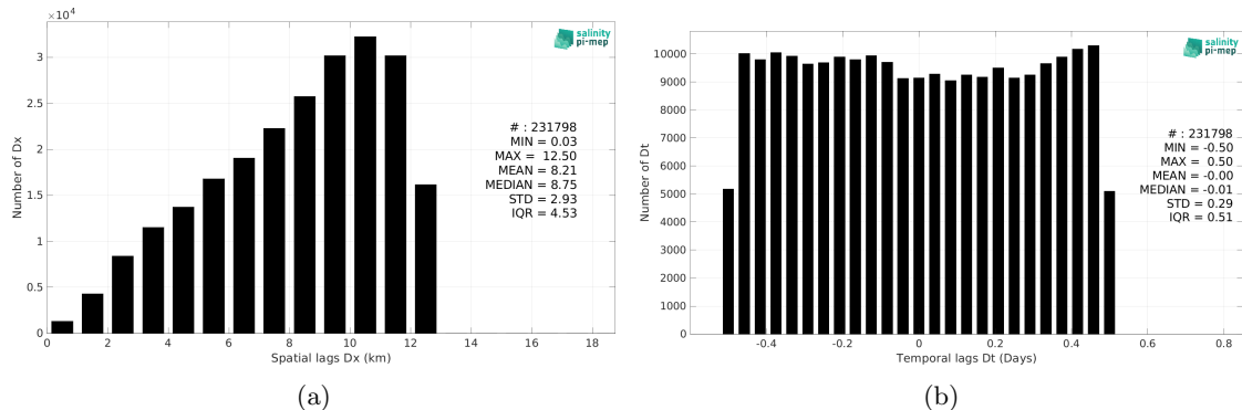
Figure 6: Histograms of the spatial (a) and temporal (b) lags between the location/time of the TSG (GOSUD-Research-vessel) measurement and the date of the corresponding SMOS SSS L3 MED-ATL-OA v2 - 9 Days (BEC) SSS pixel.
