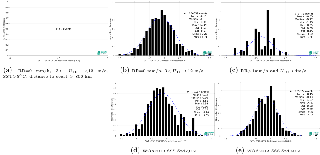
Figure 15: Normalized histogram of \Delta SSS (SMOS SSS L3 MED-ATL-OA v2 - 9 Days (BEC) - TSG (GOSUD-Research-vessel)) for 5 different subdatasets corresponding to: RR=0 mm/h, 3 < U_{10} < 12 m/s, SST > 5°C, distance to coast > 800 km (a), RR=0 mm/h, 3 < U_{10} < 12 m/s (b), RR > 1mm/h and U_{10} < 4 m/s (c), WOA2013 SSS Std < 0.2 (d), WOA2013 SSS Std > 0.2 (e).
