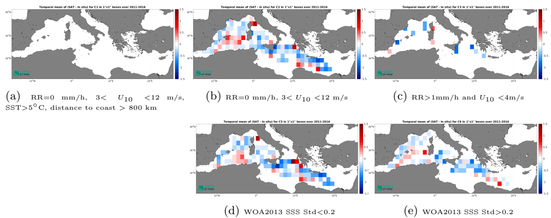
Figure 14: Temporal mean gridded over spatial boxes of size 1^\circ \times 1^\circ of \Delta SSS (SMOS SSS L3 MED-ATL-OA v2 - 9 Days (BEC) - TSG (GOSUD-Research-vessel)) for 5 different subdatasets corresponding to:RR=0 mm/h, 3 < U_{10} < 12 m/s, SST>5°C, distance to coast > 800 km (a), RR=0 mm/h, 3 < U_{10} < 12 m/s (b), RR>1mm/h and U_{10} < 4 m/s (c), WOA2013 SSS Std<0.2 (d), WOA2013 SSS Std>0.2 (e).
