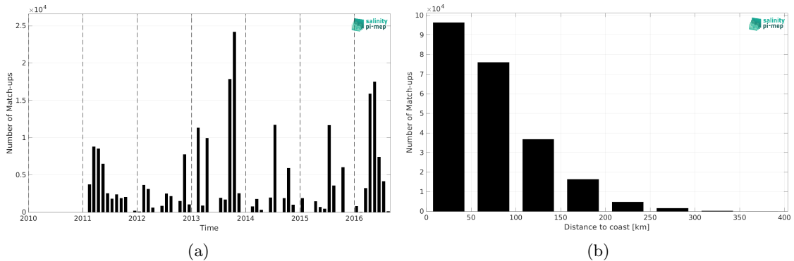
Figure 2: Number of match-ups between TSG (GOSUD-Research-vessel) and SMOS SSS L3 MED-ATL-OA v2 - 9 Days (BEC) SSS as a function of time (a) and as function of the distance to coast (b) over the Mediterranean Sea Pi-MEP region and for the full satellite product period.
