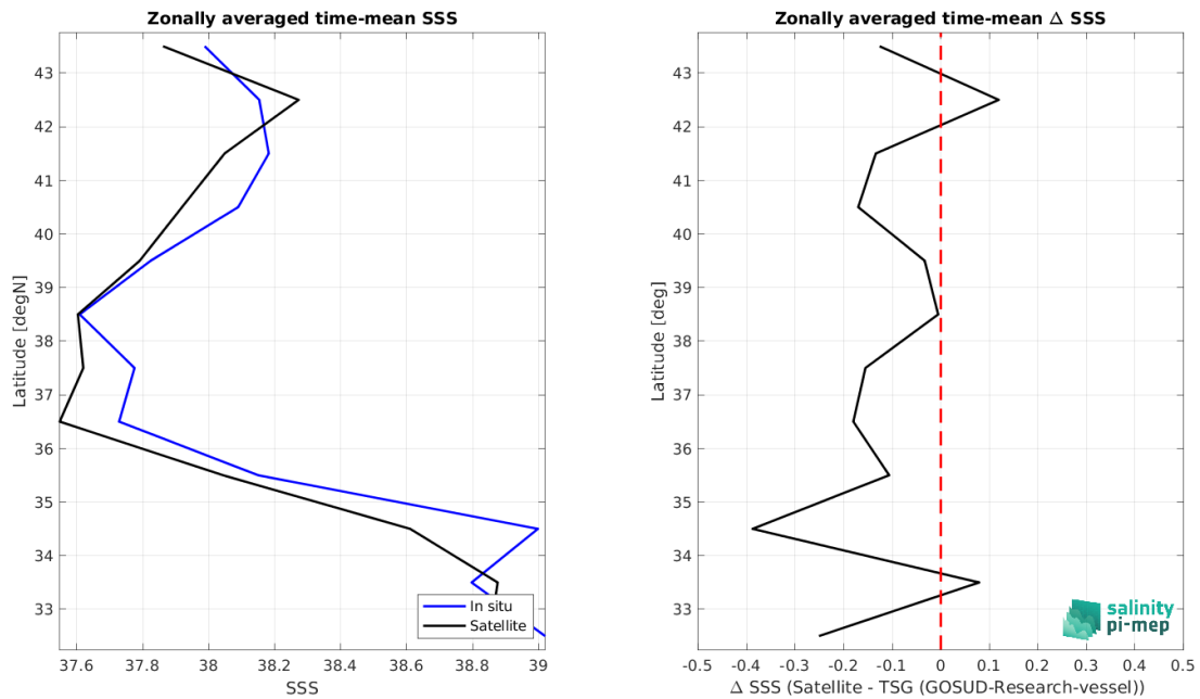
Figure 9: Left panel: Zonal mean SSS from SMOS SSS L3 MED-ATL-OA v2 - 9 Days (BEC) satellite product (black) and from TSG (GOSUD-Research-vessel) (blue). Right panel: Zonal mean of \Delta SSS (Satellite - TSG (GOSUD-Research-vessel)) for all the collected Pi-MEP match-up pairs estimated over the full satellite product period.
