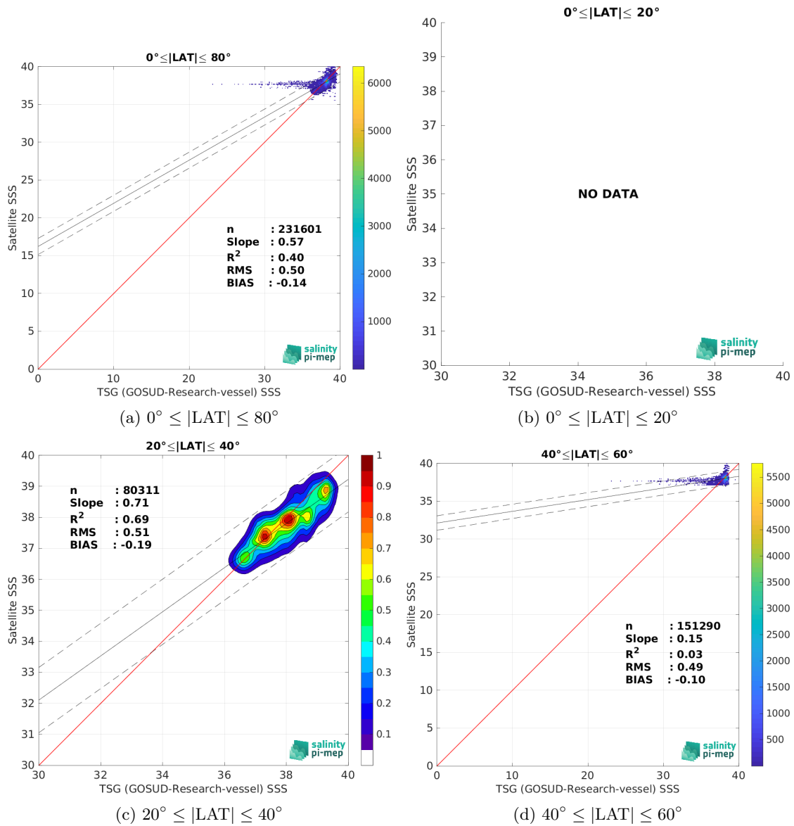
Figure 10: Contour maps of the concentration of SMOS SSS L3 MED-ATL-OA v2 - 9 Days (BEC) SSS (y-axis) versus TSG (GOSUD-Research-vessel) SSS (x-axis) at match-up pairs for different latitude bands. For each plot, the red line shows x=y . The black thin and dashed lines indicate a linear fit through the data cloud and the \pm 95\% confidence levels, respectively. The number match-up pairs n , the slope and R^2 coefficient of the linear fit, the root mean square (RMS) and the mean bias between satellite and in situ data are indicated for each latitude band in each plots.
