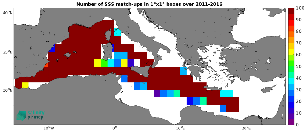
Figure 5: Number of SSS match-ups between TSG (GOSUD-Research-vessel) SSS and the SMOS SSS L3 MED-ATL-OA v2 - 9 Days (BEC) SSS product for the Mediterranean Sea Pi-MEP region over 1^\circ \times 1^\circ boxes and for the full satellite product period.
