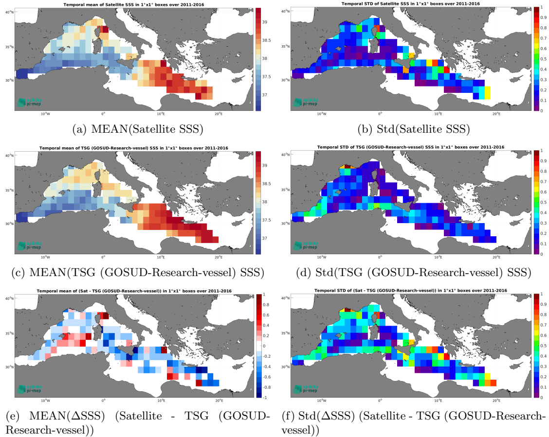
Figure 7: Temporal mean (left) and Std (right) of SSS from SMOS SSS L3 MED-ATL-OA v2 - 9 Days (BEC) (top), TSG (GOSUD-Research-vessel) (middle), and of \Delta\text{SSS} (Satellite - TSG (GOSUD-Research-vessel)). Only match-up pairs are used to generate these maps.
