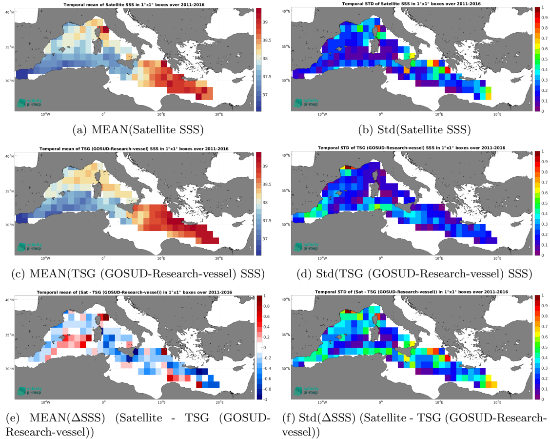
Figure 6: Temporal mean (left) and Std (right) of SSS from SMOS SSS L3 MED-ATL-OA v2 - 9 Days (BEC) (top), TSG (GOSUD-Research-vessel) (middle), and of \Delta\text{SSS} (Satellite - TSG (GOSUD-Research-vessel)). Only match-up pairs are used to generate these maps.
