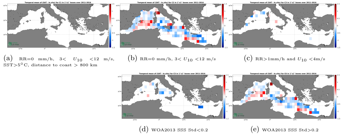
Figure 12: Temporal mean gridded over spatial boxes of size 1^\circ \times 1^\circ of \Delta SSS (SMOS SSS L3 MED-ATL-OA v2 - 9 Days (BEC) - TSG (GOSUD-Research-vessel)) for 5 different subdatasets corresponding to:RR=0 mm/h, 3 < U_{10} < 12 m/s, SST >5^\circ\text{C} , distance to coast > 800 km (a), RR=0 mm/h, 3 < U_{10} < 12 m/s (b), RR >1 mm/h and U_{10} < 4 m/s (c), WOA2013 SSS Std <0.2 (d), WOA2013 SSS Std >0.2 (e).
