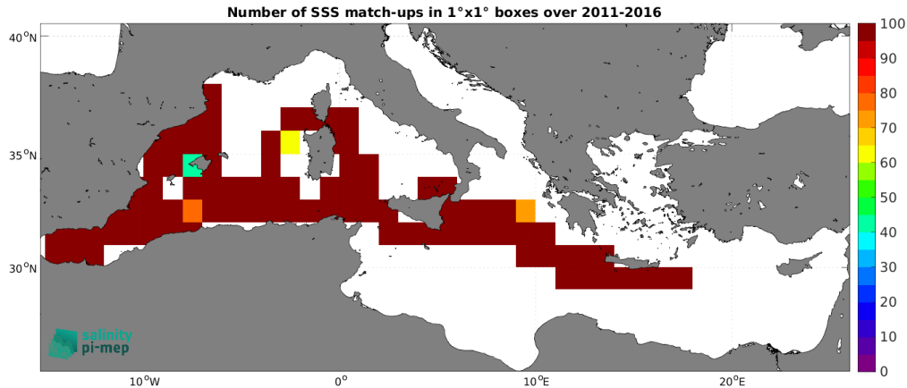
Figure 5: Number of SSS match-ups between TSG (CSIC-UTM) SSS and the SMOS SSS L3 MED-ATL-OA v2 - 9 Days (BEC) SSS product for the Mediterranean Sea Pi-MEP region over 1^\circ \times 1^\circ boxes and for the full satellite product period.
