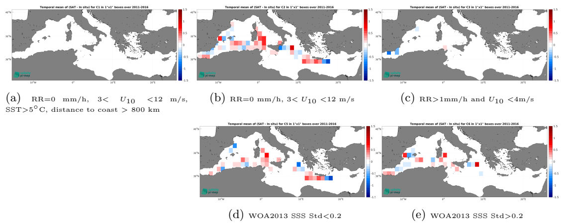
Figure 14: Temporal mean gridded over spatial boxes of size 1^\circ \times 1^\circ of \Delta\text{SSS} (SMOS SSS L3 MED-ATL-OA v2 - 9 Days (BEC) - TSG (CSIC-UTM)) for 5 different subdatasets corresponding to:RR=0 mm/h, 3 < U_{10} < 12 m/s, SST>5°C, distance to coast > 800 km (a), RR=0 mm/h, 3 < U_{10} < 12 m/s (b), RR>1mm/h and U_{10} < 4 m/s (c), WOA2013 SSS Std<0.2 (d), WOA2013 SSS Std>0.2 (e).
