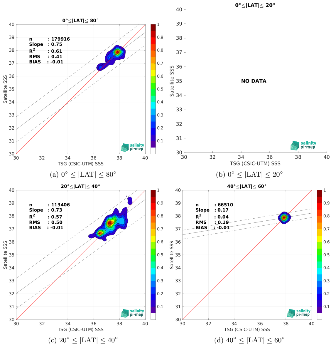
Figure 10: Contour maps of the concentration of SMOS SSS L3 MED-ATL-OA v2 - 9 Days (BEC) SSS (y-axis) versus TSG (CSIC-UTM) SSS (x-axis) at match-up pairs for different latitude bands. For each plot, the red line shows x=y . The black thin and dashed lines indicate a linear fit through the data cloud and the \pm 95\% confidence levels, respectively. The number match-up pairs n , the slope and R^2 coefficient of the linear fit, the root mean square (RMS) and the mean bias between satellite and in situ data are indicated for each latitude band in each plots.
