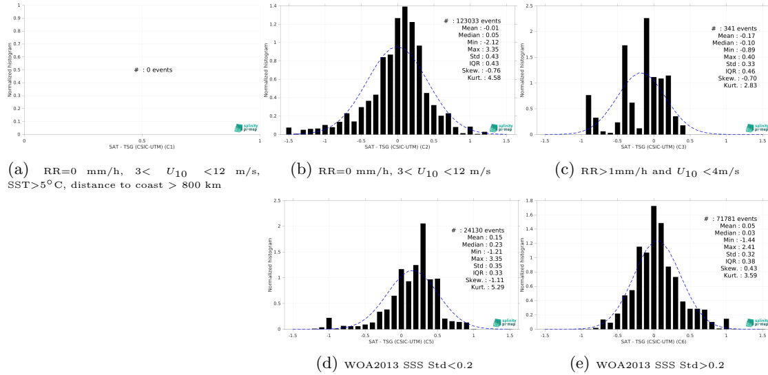
Figure 15: Normalized histogram of \Delta SSS (SMOS SSS L3 MED-ATL-OA v2 - 9 Days (BEC) - TSG (CSIC-UTM)) for 5 different subdatasets corresponding to: RR=0 mm/h, 3 < U_{10} < 12 m/s, SST > 5°C, distance to coast > 800 km (a), RR=0 mm/h, 3 < U_{10} < 12 m/s (b), RR > 1mm/h and U_{10} < 4 m/s (c), WOA2013 SSS Std < 0.2 (d), WOA2013 SSS Std > 0.2 (e).
