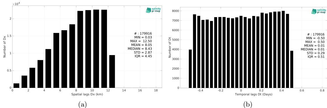
Figure 6: Histograms of the spatial (a) and temporal (b) lags between the location/time of the TSG (CSIC-UTM) measurement and the date of the corresponding SMOS SSS L3 MED-ATL-OA v2 - 9 Days (BEC) SSS pixel.
