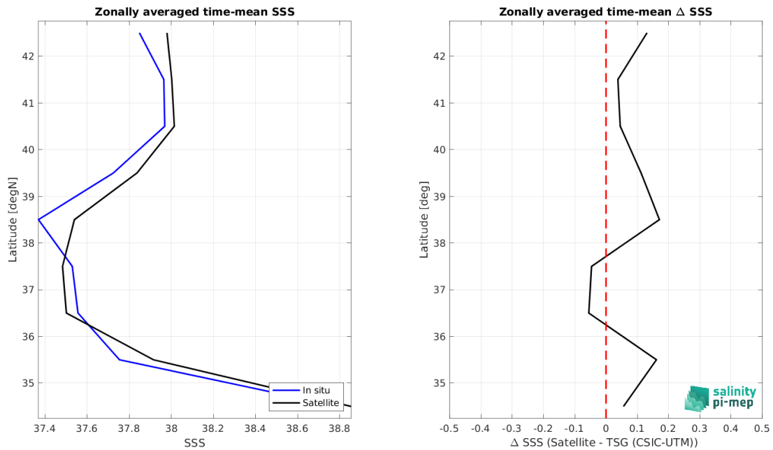
Figure 9: Left panel: Zonal mean SSS from SMOS SSS L3 MED-ATL-OA v2 - 9 Days (BEC) satellite product (black) and from TSG (CSIC-UTM) (blue). Right panel: Zonal mean of \Delta SSS (Satellite - TSG (CSIC-UTM)) for all the collected Pi-MEP match-up pairs estimated over the full satellite product period.
