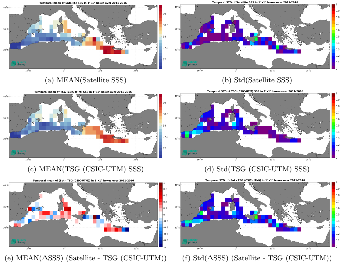
Figure 7: Temporal mean (left) and Std (right) of SSS from SMOS SSS L3 MED-ATL-OA v2 - 9 Days (BEC) (top), TSG (CSIC-UTM) (middle), and of \Delta\text{SSS} (Satellite - TSG (CSIC-UTM)). Only match-up pairs are used to generate these maps.
