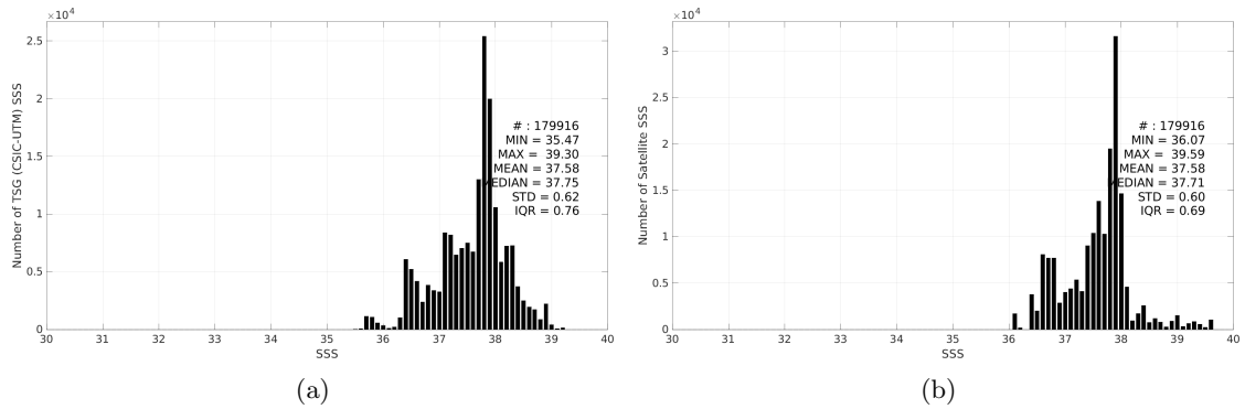
Figure 3: Histograms of SSS from TSG (CSIC-UTM) (a) and SMOS SSS L3 MED-ATL-OA v2 - 9 Days (BEC) (b) considering all match-up pairs per bins of 0.1 over the Mediterranean Sea Pi-MEP region and for the full satellite product period.
