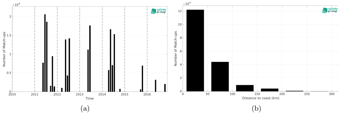
Figure 2: Number of match-ups between TSG (CSIC-UTM) and SMOS SSS L3 MED-ATL-OA v2 - 9 Days (BEC) SSS as a function of time (a) and as function of the distance to coast (b) over the Mediterranean Sea Pi-MEP region and for the full satellite product period.
