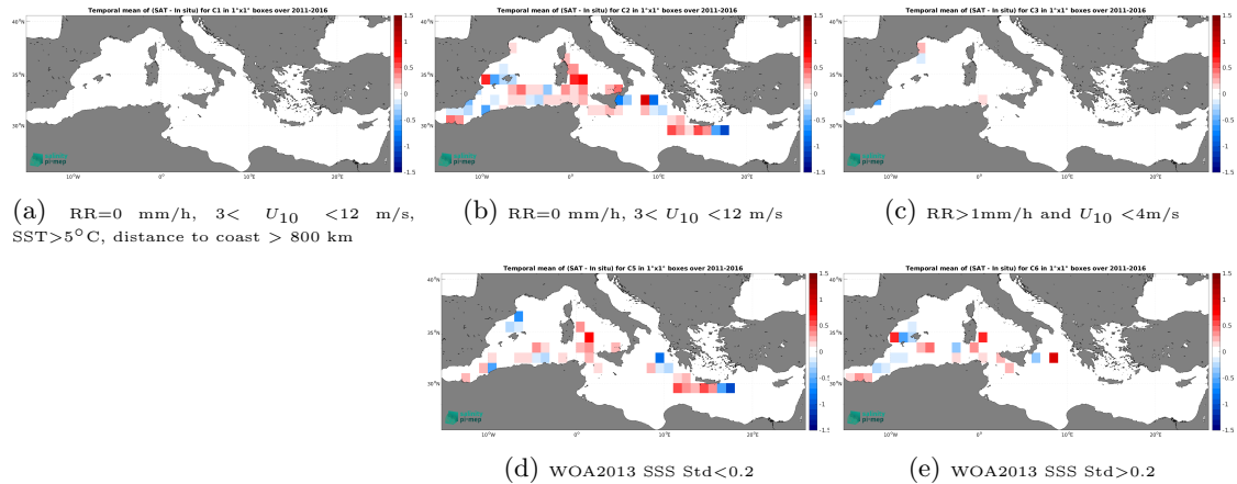
Figure 12: Temporal mean gridded over spatial boxes of size 1^\circ \times 1^\circ of \Delta\text{SSS} (SMOS SSS L3 MED-ATL-OA v2 - 9 Days (BEC) - TSG (CSIC-UTM)) for 5 different subdatasets corresponding to:RR=0 mm/h, 3 < U_{10} < 12 m/s, SST >5^\circ\text{C} , distance to coast > 800 km (a), RR=0 mm/h, 3 < U_{10} < 12 m/s (b), RR >1 mm/h and U_{10} < 4 m/s (c), WOA2013 SSS Std <0.2 (d), WOA2013 SSS Std >0.2 (e).
