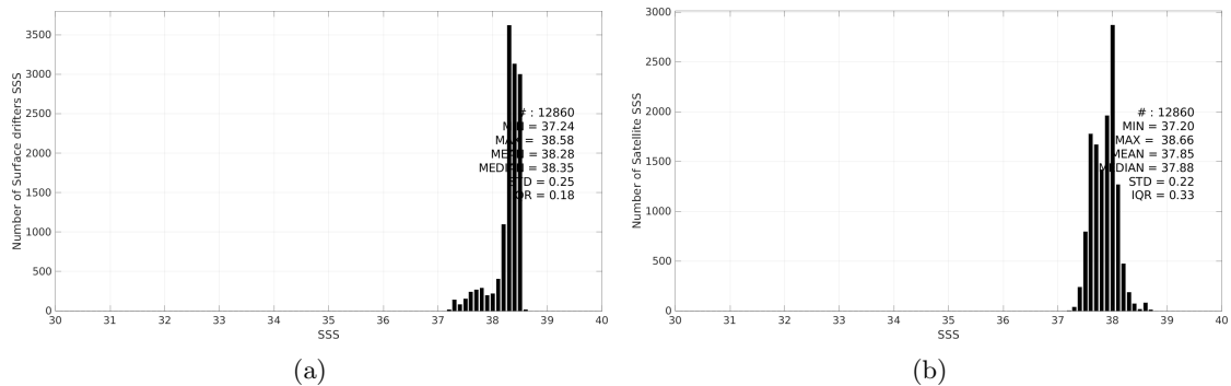
Figure 3: Histograms of SSS from Surface drifters (a) and SMOS SSS L3 MED-ATL-OA v2 - 9 Days (BEC) (b) considering all match-up pairs per bins of 0.1 over the Mediterranean Sea Pi-MEP region and for the full satellite product period.
