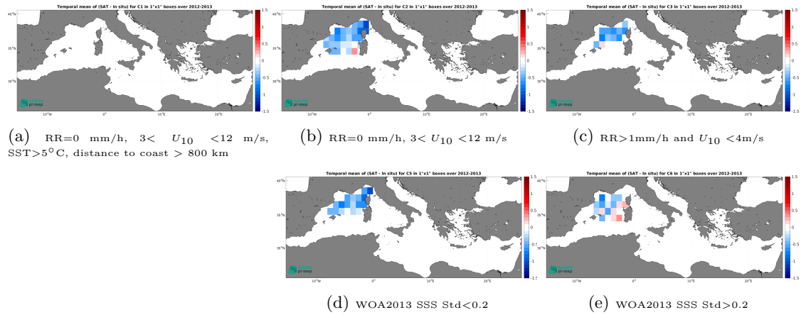
Figure 13: Temporal mean gridded over spatial boxes of size 1^\circ \times 1^\circ of \Delta SSS (SMOS SSS L3 MED-ATL-OA v2 - 9 Days (BEC) - Surface drifters) for 5 different subdatasets corresponding to:RR=0 mm/h, 3 < U_{10} < 12 m/s, SST >5^\circ\text{C} , distance to coast > 800 km (a), RR=0 mm/h, 3 < U_{10} < 12 m/s (b), RR >1 mm/h and U_{10} < 4 m/s (c), WOA2013 SSS Std <0.2 (d), WOA2013 SSS Std >0.2 (e).
