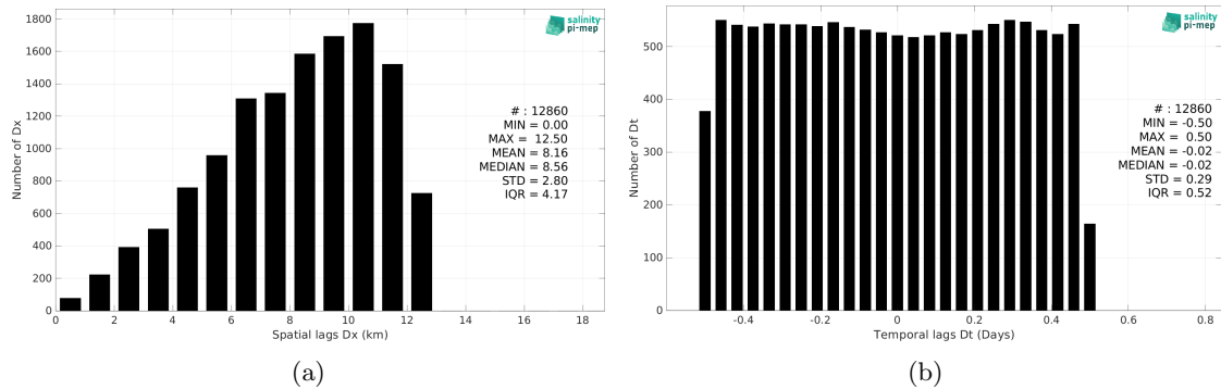
Figure 5: Histograms of the spatial (a) and temporal (b) lags between the location/time of the Surface drifters measurement and the date of the corresponding SMOS SSS L3 MED-ATL-OA v2 - 9 Days (BEC) SSS pixel.
