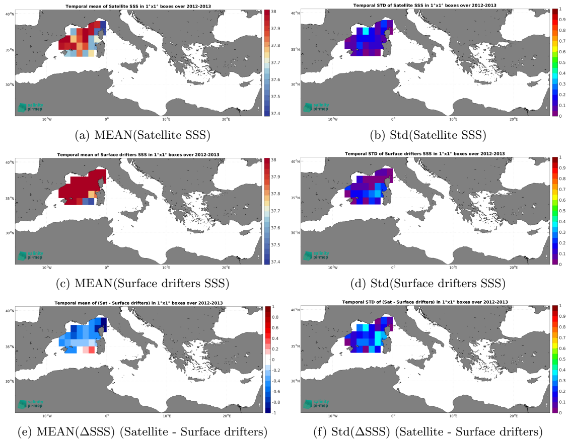
Figure 6: Temporal mean (left) and Std (right) of SSS from SMOS SSS L3 MED-ATL-OA v2 - 9 Days (BEC) (top), Surface drifters (middle), and of \Delta SSS (Satellite - Surface drifters). Only match-up pairs are used to generate these maps.
