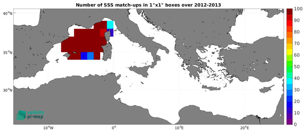
Figure 4: Number of SSS match-ups between Surface drifters SSS and the SMOS SSS L3 MED-ATL-OA v2 - 9 Days (BEC) SSS product for the Mediterranean Sea Pi-MEP region over 1^\circ \times 1^\circ boxes and for the full satellite product period.
