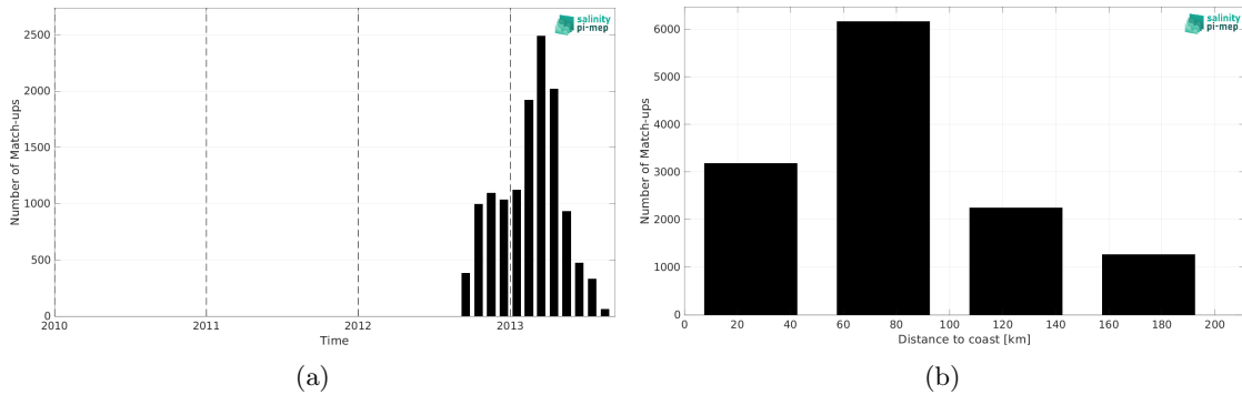
Figure 2: Number of match-ups between Surface drifters and SMOS SSS L3 MED-ATL-OA v2 - 9 Days (BEC) SSS as a function of time (a) and as function of the distance to coast (b) over the Mediterranean Sea Pi-MEP region and for the full satellite product period.
