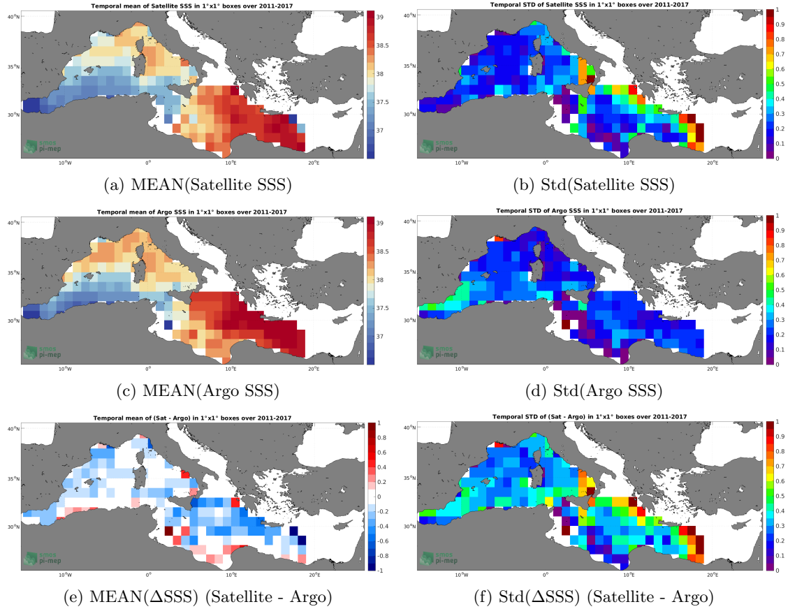
Figure 6: Temporal mean (left) and Std (right) of SSS from SMOS SSS L3 MED-ATL-OA v2 - 9 Days (BEC) (top), Argo (middle), and of \Delta\text{SSS} (Satellite - Argo). Only match-up pairs are used to generate these maps.
