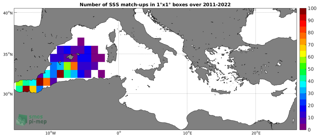
Figure 4: Number of SSS match-ups between Argo SSS and the SMOS SSS L2-AVERAGED v700 (ESA) SSS product for the Mediterranean Sea Pi-MEP region over 1^\circ \times 1^\circ boxes and for the full satellite product period.
