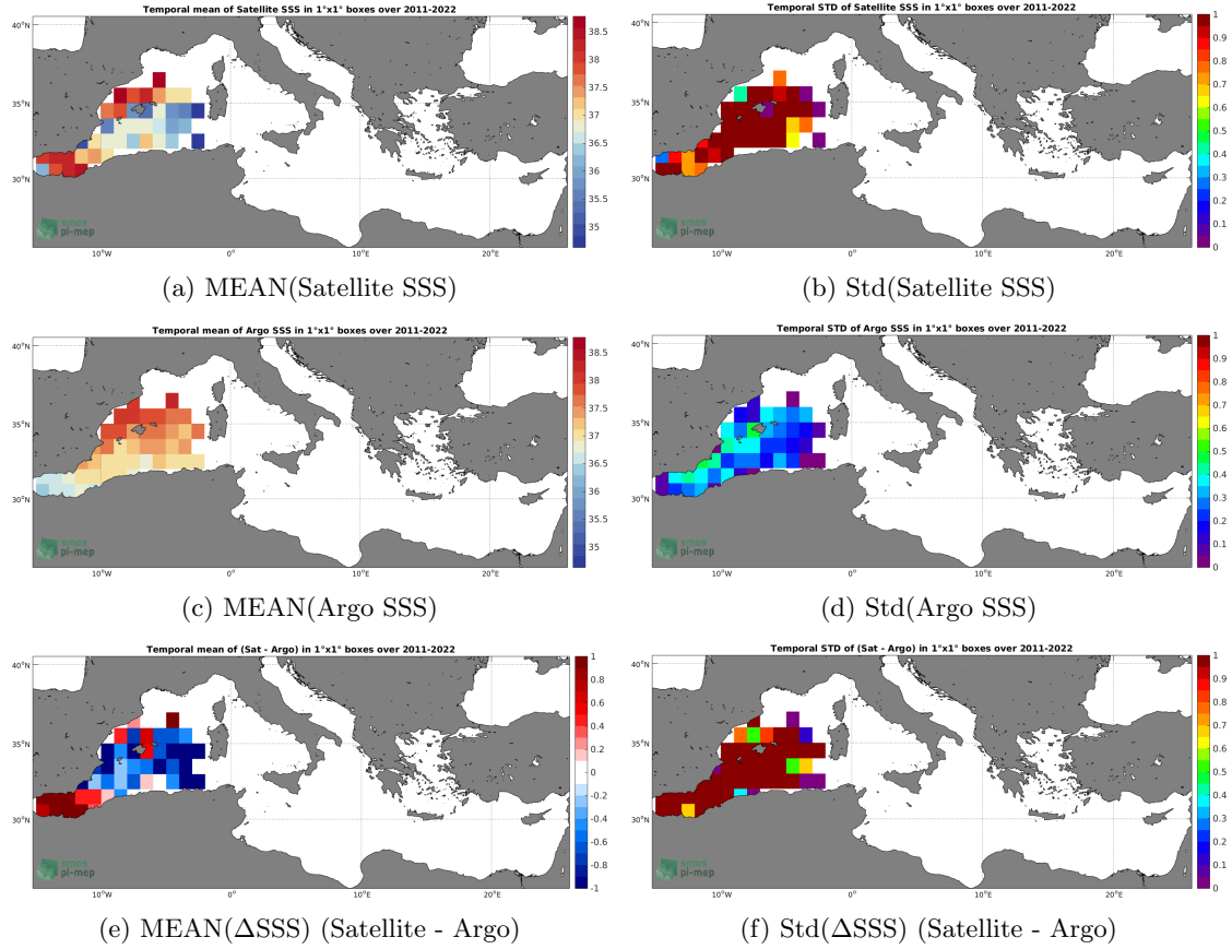
Figure 6: Temporal mean (left) and Std (right) of SSS from SMOS SSS L2-AVERAGED v700 (ESA) (top), Argo (middle), and of \Delta SSS (Satellite - Argo). Only match-up pairs are used to generate these maps.
