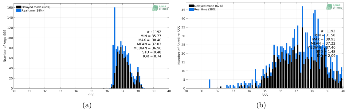
Figure 2: Histograms of SSS from Argo (a) and SMOS SSS L2-AVERAGED v700 (ESA) (b) considering all match-up pairs per bins of 0.1 over the Mediterranean Sea Pi-MEP region and for the full satellite product period.
