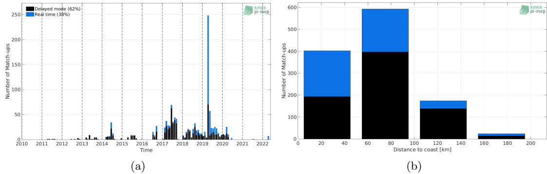
Figure 1: Number of match-ups between Argo and SMOS SSS L2-AVERAGED v700 (ESA) SSS as a function of time (a) and as function of the distance to coast (b) over the Mediterranean Sea Pi-MEP region and for the full satellite product period.
