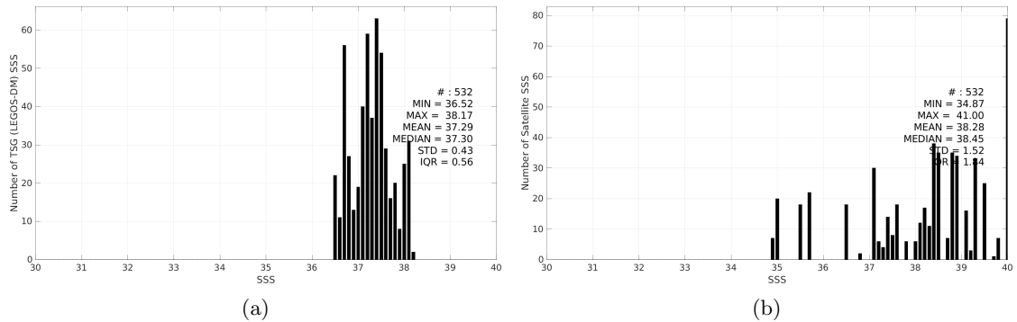
Figure 3: Histograms of SSS from TSG (LEGOS-DM) (a) and SMOS SSS L2 v700 (ESA) (b) considering all match-up pairs per bins of 0.1 over the Mediterranean Sea Pi-MEP region and for the full satellite product period.
