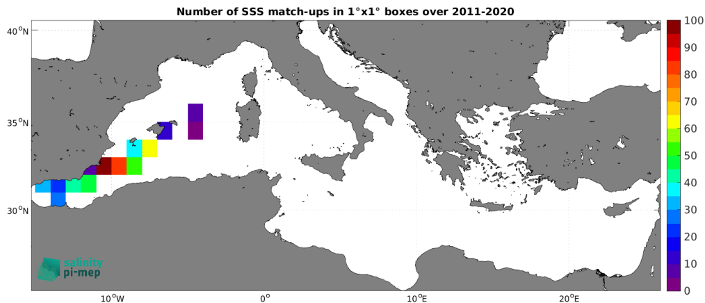
Figure 5: Number of SSS match-ups between TSG (LEGOS-DM) SSS and the SMOS SSS L2 v700 (ESA) SSS product for the Mediterranean Sea Pi-MEP region over 1^\circ \times 1^\circ boxes and for the full satellite product period.
