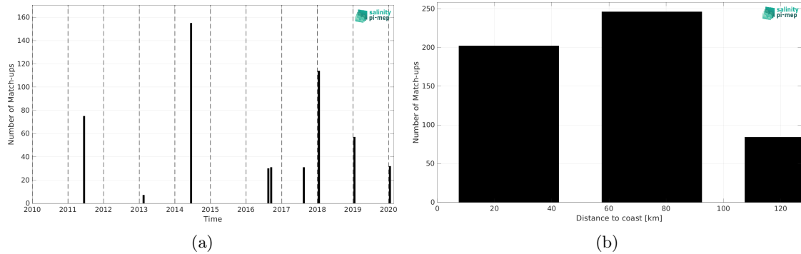
Figure 2: Number of match-ups between TSG (LEGOS-DM) and SMOS SSS L2 v700 (ESA) SSS as a function of time (a) and as function of the distance to coast (b) over the Mediterranean Sea Pi-MEP region and for the full satellite product period.
