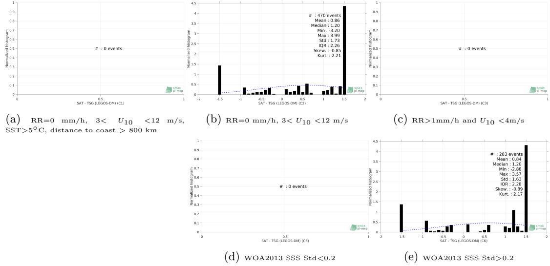
Figure 13: Normalized histogram of \Delta\text{SSS} (SMOS SSS L2 v700 (ESA) - TSG (LEGOS-DM)) for 5 different subdatasets corresponding to: RR=0 mm/h, 3 < U_{10} < 12 m/s, SST > 5^\circ\text{C} , distance to coast > 800 km (a), RR=0 mm/h, 3 < U_{10} < 12 m/s (b), RR > 1\text{mm/h} and U_{10} < 4\text{m/s} (c), WOA2013 SSS Std < 0.2 (d), WOA2013 SSS Std > 0.2 (e).
