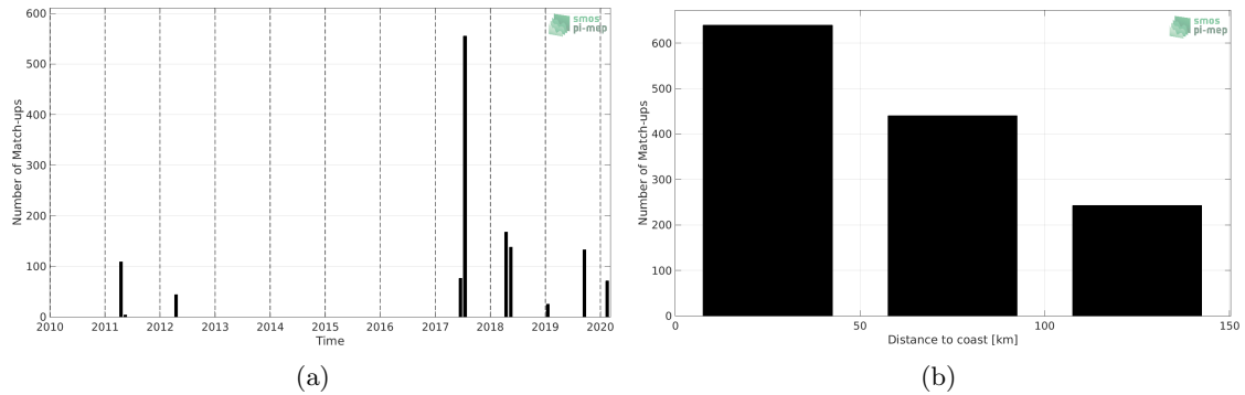
Figure 1: Number of match-ups between TSG (GOSUD-Research-vessel) and SMOS SSS L2 v700 (ESA) SSS as a function of time (a) and as function of the distance to coast (b) over the Mediterranean Sea Pi-MEP region and for the full satellite product period.
