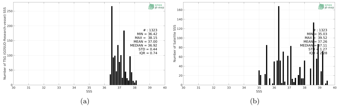
Figure 2: Histograms of SSS from TSG (GOSUD-Research-vessel) (a) and SMOS SSS L2 v700 (ESA) (b) considering all match-up pairs per bins of 0.1 over the Mediterranean Sea Pi-MEP region and for the full satellite product period.
