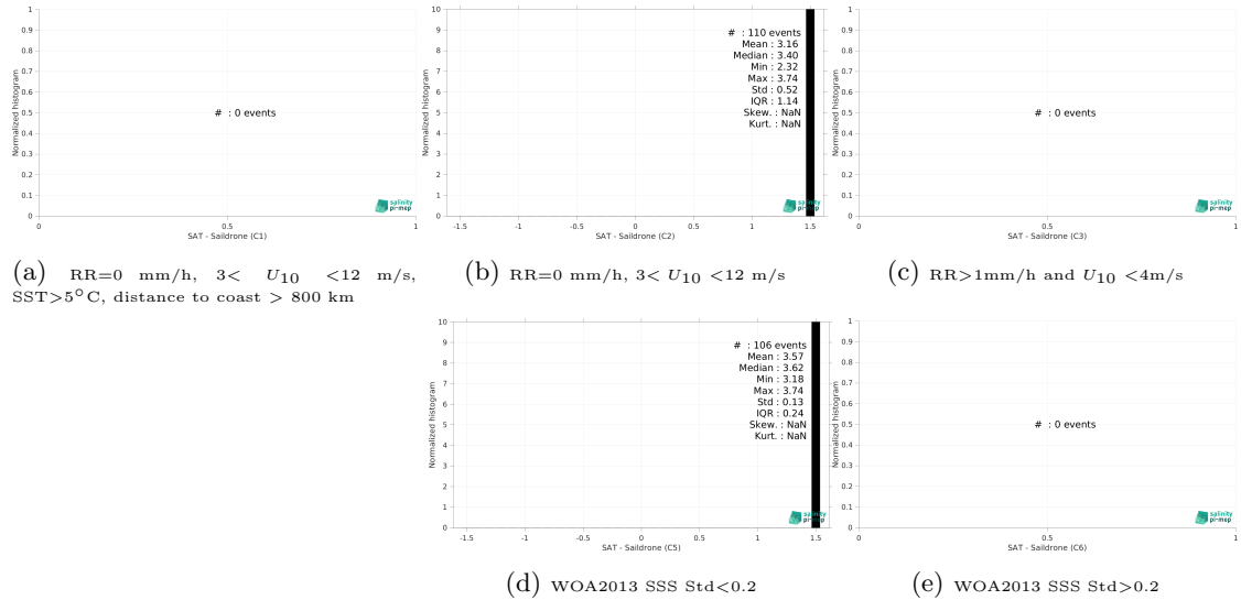
Figure 15: Normalized histogram of \Delta SSS (SMOS SSS L2 v700 (ESA) - Saldrone) for 5 different subdatasets corresponding to: RR=0 mm/h, 3 < U_{10} < 12 m/s, SST > 5°C, distance to coast > 800 km (a), RR=0 mm/h, 3 < U_{10} < 12 m/s (b), RR > 1mm/h and U_{10} < 4 m/s (c), WOA2013 SSS Std < 0.2 (d), WOA2013 SSS Std > 0.2 (e).
