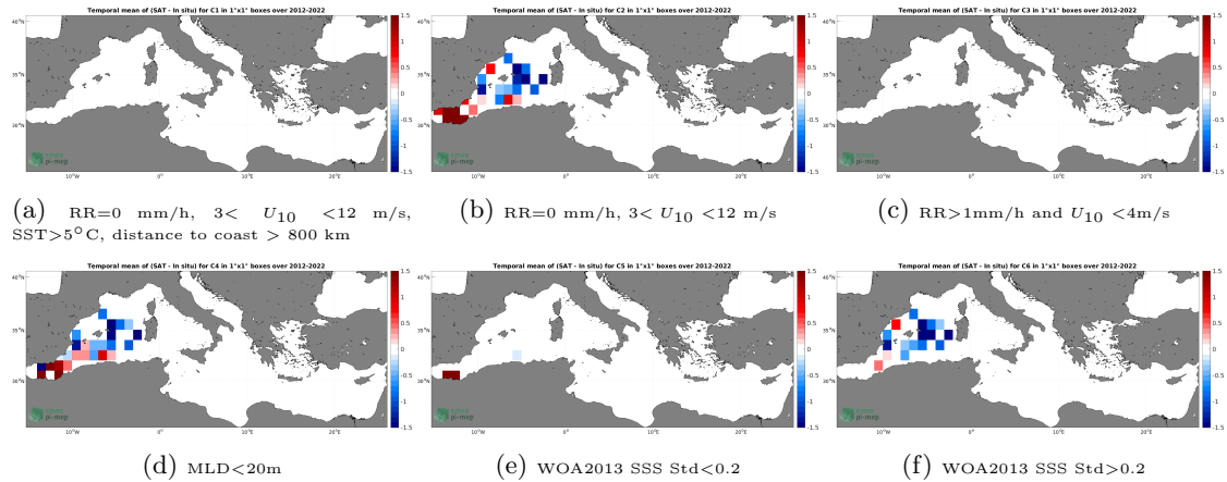
Figure 12: Temporal mean gridded over spatial boxes of size 1^{\circ}\times 1^{\circ} of \Delta\text{SSS} (SMOS SSS L2 v700 (ESA) - Argo) for 6 different subdatasets corresponding to:RR=0 mm/h, 3 < U_{10} < 12 m/s, SST >5^{\circ}\text{C} , distance to coast > 800 km (a), RR=0 mm/h, 3 < U_{10} < 12 m/s (b), RR >1\text{mm/h} and U_{10} < 4\text{m/s} (c),MLD <20\text{m} (d),WOA2013 SSS Std <0.2 (e),WOA2013 SSS Std >0.2 (f).
