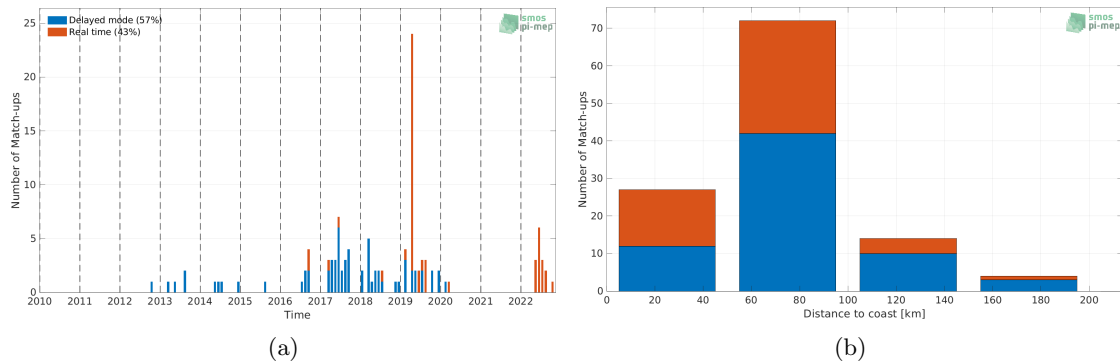
Figure 1: Number of match-ups between Argo and SMOS SSS L2 v700 (ESA) SSS as a function of time (a) and as function of the distance to coast (b) over the Mediterranean Sea Pi-MEP region and for the full satellite product period.
