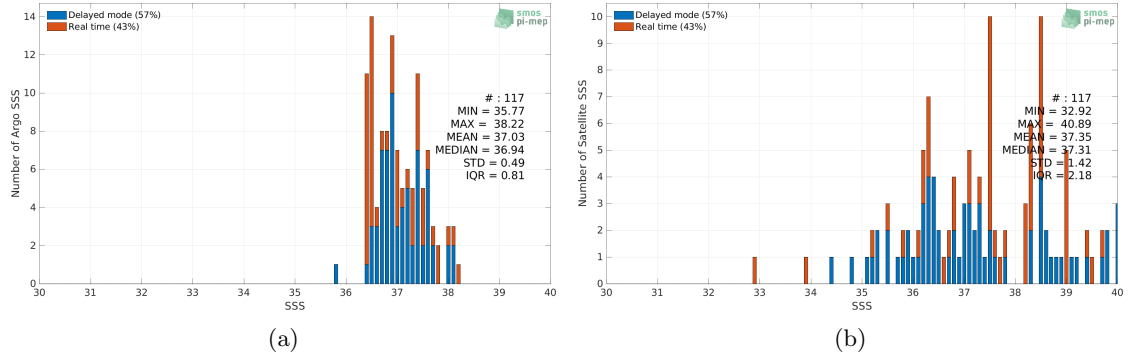
Figure 2: Histograms of SSS from Argo (a) and SMOS SSS L2 v700 (ESA) (b) considering all match-up pairs per bins of 0.1 over the Mediterranean Sea Pi-MEP region and for the full satellite product period.
