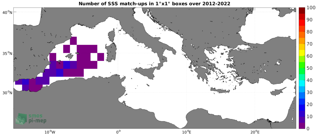
Figure 4: Number of SSS match-ups between Argo SSS and the SMOS SSS L2 v700 (ESA) SSS product for the Mediterranean Sea Pi-MEP region over 1^\circ \times 1^\circ boxes and for the full satellite product period.
