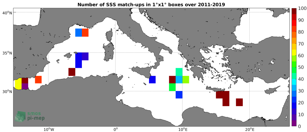
Figure 4: Number of SSS match-ups between TSG (GOSUD-Research-vessel) SSS and the SMOS SSS L2 v662 (ESA) SSS product for the Mediterranean Sea Pi-MEP region over 1^\circ \times 1^\circ boxes and for the full satellite product period.
