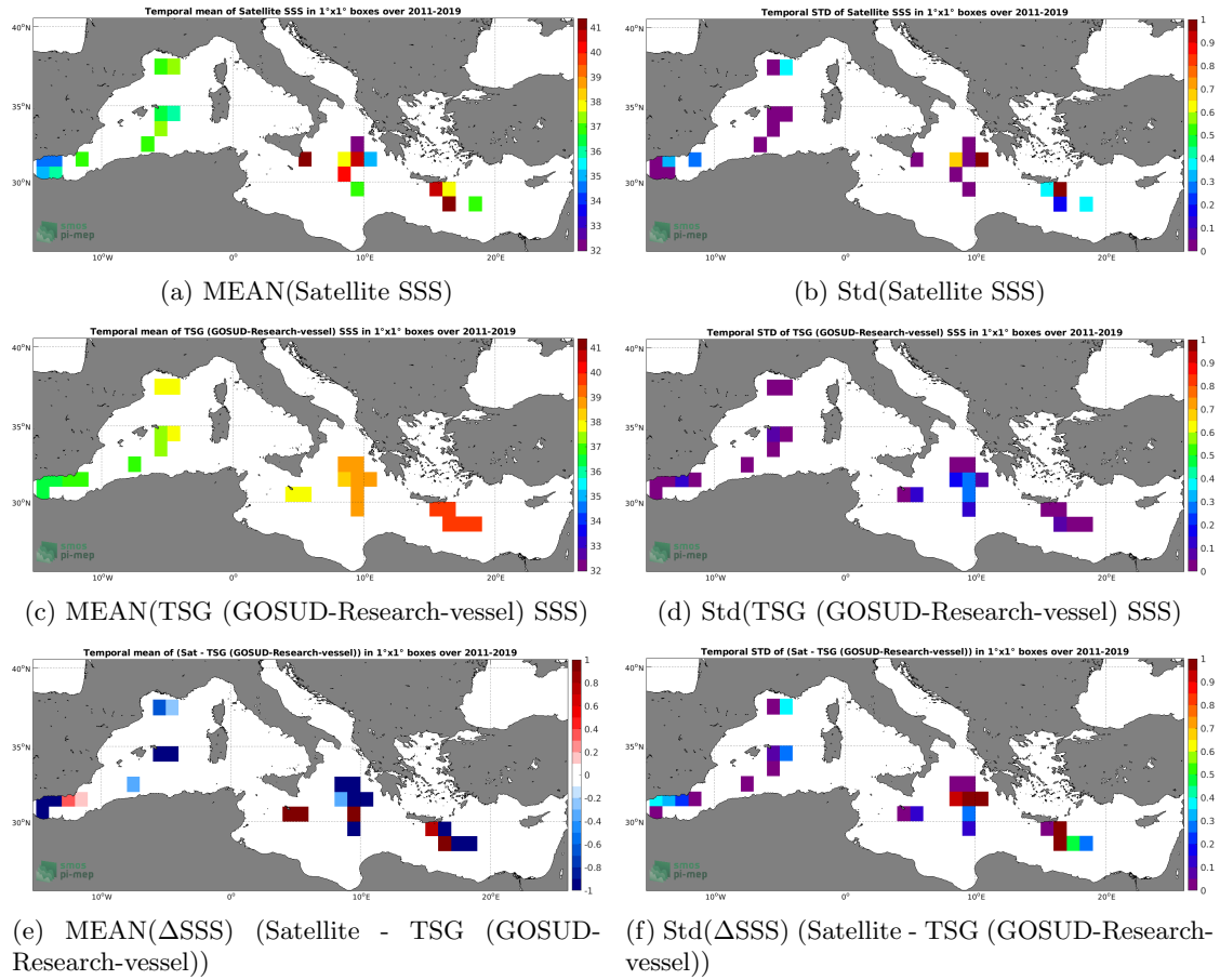
Figure 6: Temporal mean (left) and Std (right) of SSS from SMOS SSS L2 v662 (ESA) (top), TSG (GOSUD-Research-vessel) (middle), and of \Delta SSS (Satellite - TSG (GOSUD-Research-vessel)). Only match-up pairs are used to generate these maps.
