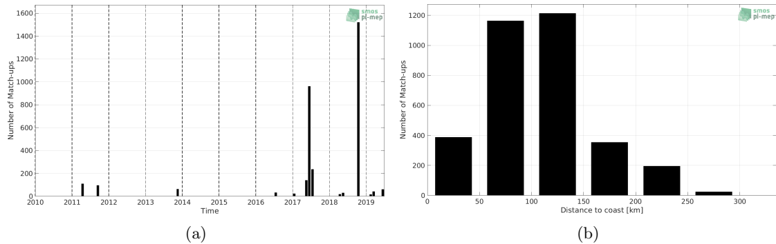
Figure 1: Number of match-ups between TSG (GOSUD-Research-vessel) and SMOS SSS L2 v662 (ESA) SSS as a function of time (a) and as function of the distance to coast (b) over the Mediterranean Sea Pi-MEP region and for the full satellite product period.
