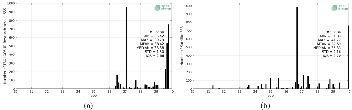
Figure 2: Histograms of SSS from TSG (GOSUD-Research-vessel) (a) and SMOS SSS L2 v662 (ESA) (b) considering all match-up pairs per bins of 0.1 over the Mediterranean Sea Pi-MEP region and for the full satellite product period.
