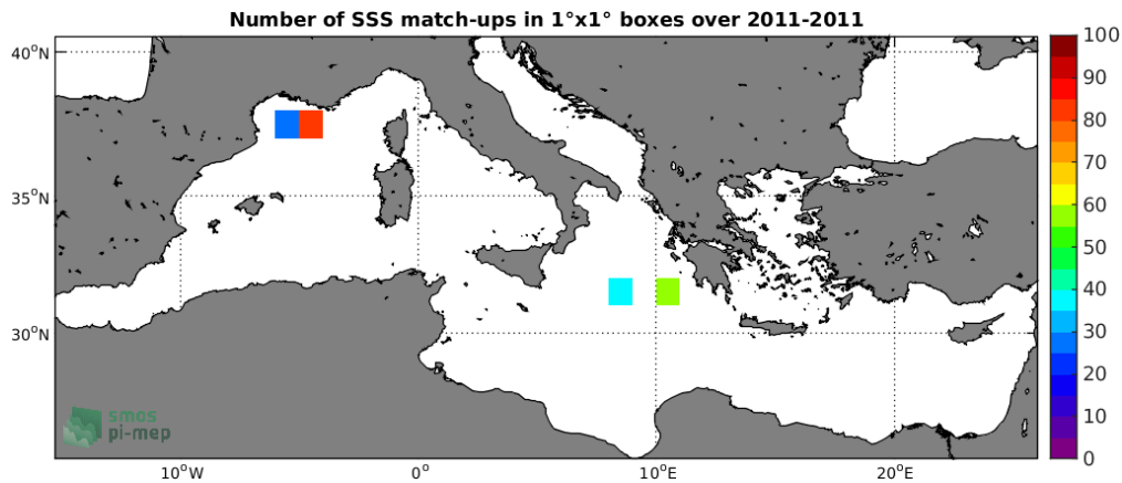
Figure 4: Number of SSS match-ups between TSG-GOSUD-Research-vessel SSS and the SMOS-L2-DPGS-v662 SSS product for the Mediterranean Sea Pi-MEP region over 1°x1° boxes and for the full satellite product period.
