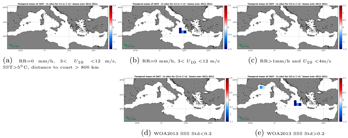
Figure 12: Temporal mean gridded over spatial boxes of size 1^\circ \times 1^\circ of \Delta SSS (SMOS-L2-DPGS-v662 - TSG-GOSUD-Research-vessel) for 5 different subdatasets corresponding to:RR=0 mm/h, 3 < U_{10} < 12 m/s, SST>5°C, distance to coast > 800 km (a), RR=0 mm/h, 3 < U_{10} < 12 m/s (b), RR>1mm/h and U_{10} < 4 m/s (c), WOA2013 SSS Std<0.2 (d), WOA2013 SSS Std>0.2 (e).
