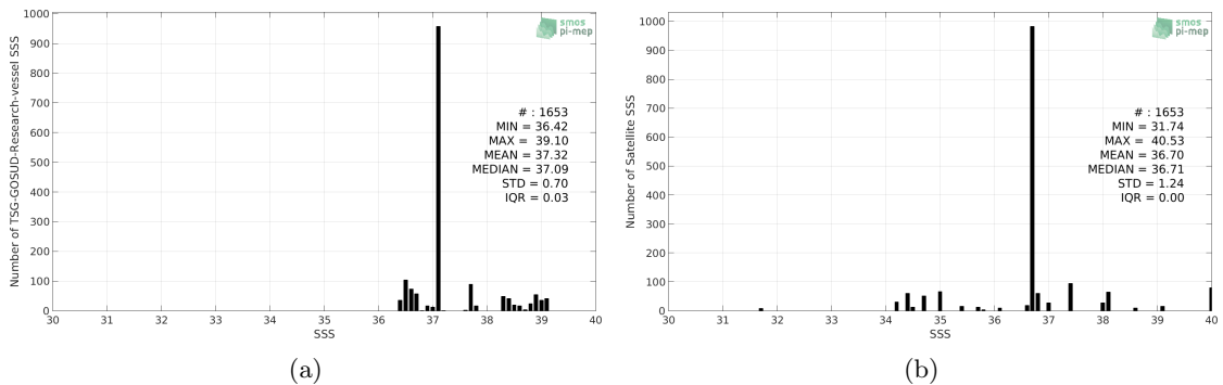
Figure 2: Histograms of SSS from TSG-GOSUD-Research-vessel (a) and SMOS-L2-DPGS-v662 (b) considering all match-up pairs per bins of 0.1 over the Mediterranean Sea Pi-MEP region and for the full satellite product period.
