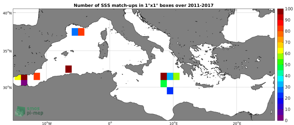
Figure 4: Number of SSS match-ups between TSG-GOSUD-Research-vessel SSS and the SMOS-L2-DPGS-v662 SSS product for the Mediterranean Sea Pi-MEP region over 1^\circ \times 1^\circ boxes and for the full satellite product period.
