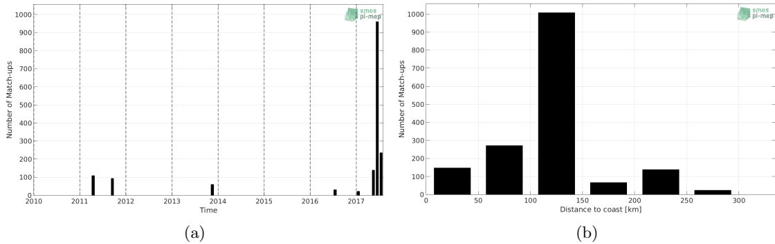
Figure 1: Number of match-ups between TSG-GOSUD-Research-vessel and SMOS-L2-DPGS-v662 SSS as a function of time (a) and as function of the distance to coast (b) over the Mediterranean Sea Pi-MEP region and for the full satellite product period.
