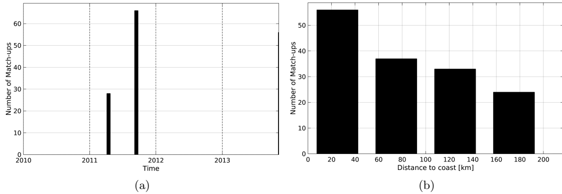
Figure 1: Number of match-ups between TSG-GOSUD-Research-vessel and SMOS-L2-DPGS-v662 SSS as a function of time (a) and as function of the distance to coast (b) over the Mediterranean Sea Pi-MEP region and for the full satellite product period.
