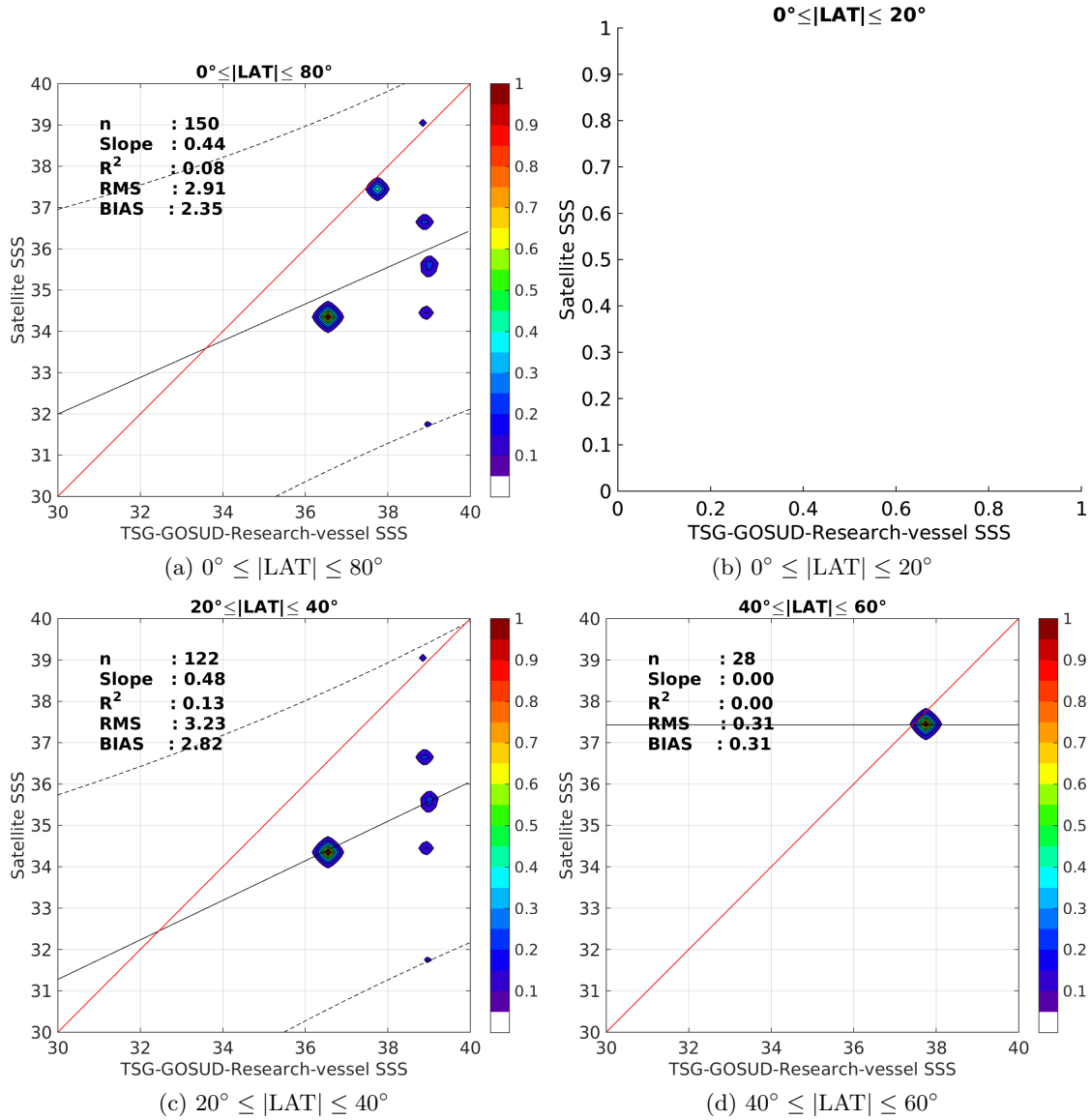
Figure 9: Contour maps of the concentration of SMOS-L2-DPGS-v662 SSS ( y -axis) versus TSG-GOSUD-Research-vessel SSS ( x -axis) at match-up pairs for different latitude bands. For each plot, the red line shows x=y . The black thin and dashed lines indicate a linear fit through the data cloud and the \pm 95\% confidence levels, respectively. The number match-up pairs n , the slope and R^2 coefficient of the linear fit, the root mean square (RMS) and the mean bias between satellite and in situ data are indicated for each latitude band in each plots.
