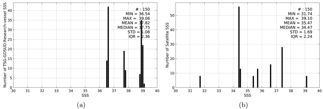
Figure 2: Histograms of SSS from TSG-GOSUD-Research-vessel (a) and SMOS-L2-DPGS-v662 (b) considering all match-up pairs per bins of 0.1 over the Mediterranean Sea Pi-MEP region and for the full satellite product period.
