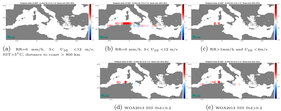
Figure 14: Temporal mean gridded over spatial boxes of size 1^\circ \times 1^\circ of \Delta SSS (SMAP SSS L4 OI v3 - Monthly (ESR) - TSG (SAMOS)) for 5 different subdatasets corresponding to:RR=0 mm/h, 3 < U_{10} < 12 m/s, SST >5^\circ\text{C} , distance to coast > 800 km (a), RR=0 mm/h, 3 < U_{10} < 12 m/s (b), RR >1 mm/h and U_{10} < 4 m/s (c), WOA2013 SSS Std <0.2 (d), WOA2013 SSS Std >0.2 (e).
