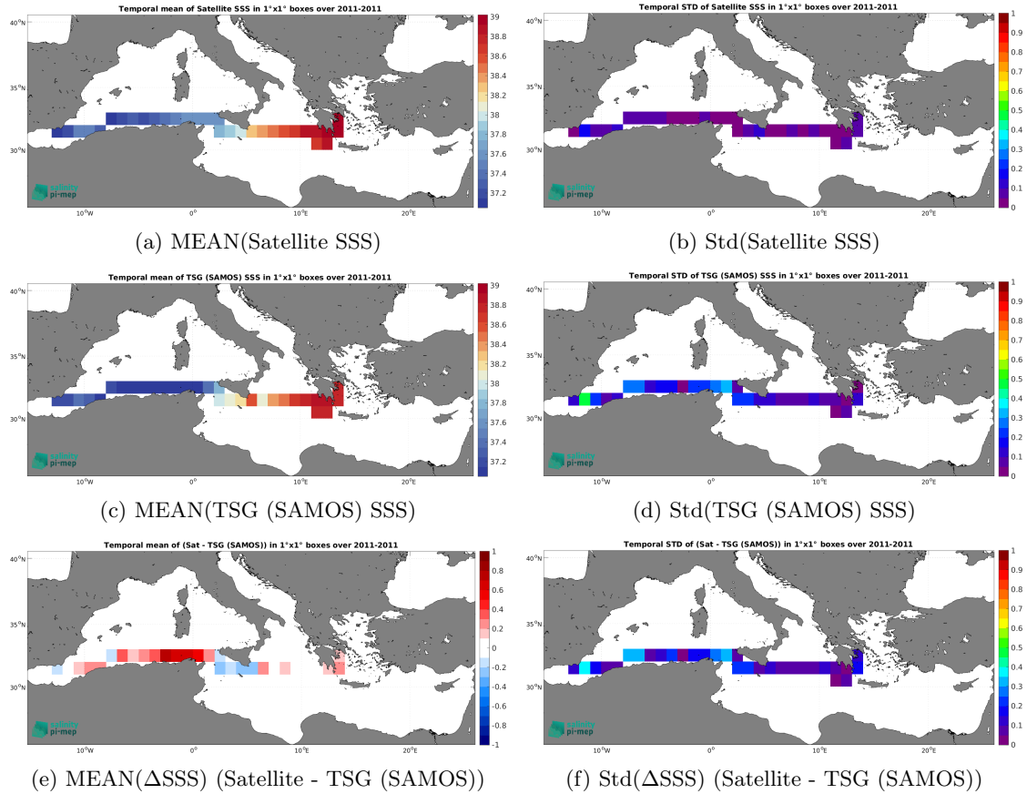
Figure 7: Temporal mean (left) and Std (right) of SSS from SMAP SSS L4 OI v3 - Monthly (ESR) (top), TSG (SAMOS) (middle), and of \Delta\text{SSS} (Satellite - TSG (SAMOS)). Only match-up pairs are used to generate these maps.
