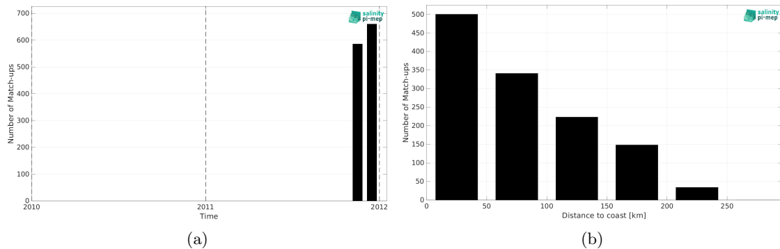
Figure 2: Number of match-ups between TSG (SAMOS) and SMAP SSS L4 OI v3 - Monthly (ESR) SSS as a function of time (a) and as function of the distance to coast (b) over the Mediterranean Sea Pi-MEP region and for the full satellite product period.
