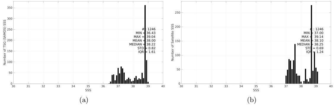
Figure 3: Histograms of SSS from TSG (SAMOS) (a) and SMAP SSS L4 OI v3 - Monthly (ESR) (b) considering all match-up pairs per bins of 0.1 over the Mediterranean Sea Pi-MEP region and for the full satellite product period.
