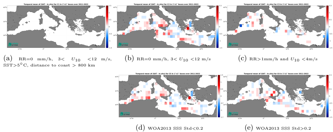
Figure 14: Temporal mean gridded over spatial boxes of size 1^\circ \times 1^\circ of \Delta\text{SSS} (SMAP SSS L4 OI v3 - Monthly (ESR) - TSG (GOSUD-Research-vessel)) for 5 different subdatasets corresponding to:RR=0 mm/h, 3 < U_{10} < 12 m/s, SST>5°C, distance to coast > 800 km (a), RR=0 mm/h, 3 < U_{10} < 12 m/s (b), RR>1mm/h and U_{10} < 4 m/s (c), WOA2013 SSS Std<0.2 (d), WOA2013 SSS Std>0.2 (e).
