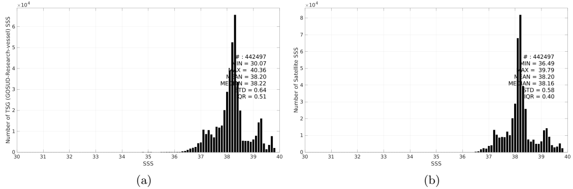
Figure 3: Histograms of SSS from TSG (GOSUD-Research-vessel) (a) and SMAP SSS L4 OI v3 - Monthly (ESR) (b) considering all match-up pairs per bins of 0.1 over the Mediterranean Sea Pi-MEP region and for the full satellite product period.
