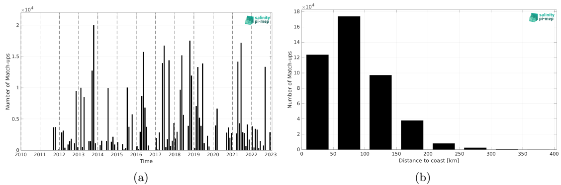
Figure 2: Number of match-ups between TSG (GOSUD-Research-vessel) and SMAP SSS L4 OI v3 - Monthly (ESR) SSS as a function of time (a) and as function of the distance to coast (b) over the Mediterranean Sea Pi-MEP region and for the full satellite product period.
