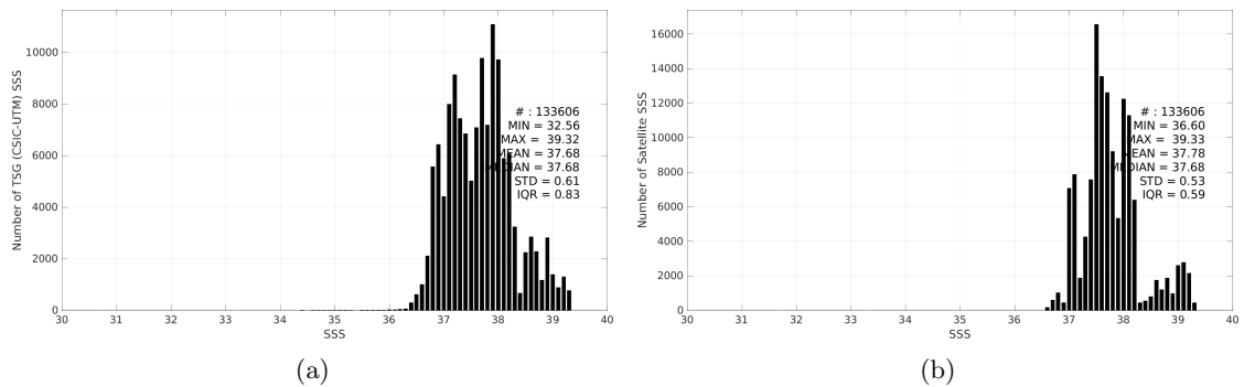
Figure 3: Histograms of SSS from TSG (CSIC-UTM) (a) and SMAP SSS L4 OI v3 - Monthly (ESR) (b) considering all match-up pairs per bins of 0.1 over the Mediterranean Sea Pi-MEP region and for the full satellite product period.
