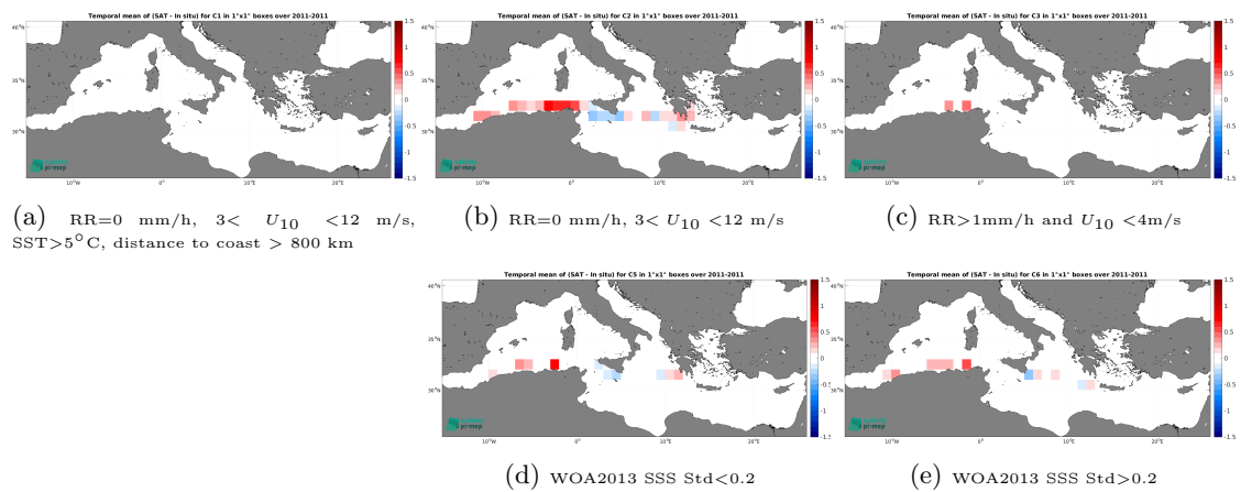
Figure 14: Temporal mean gridded over spatial boxes of size 1^\circ \times 1^\circ of \Delta\text{SSS} (SMAP SSS L4 OI v3 - Daily (ESR) - TSG (SAMOS)) for 5 different subdatasets corresponding to:RR=0 mm/h, 3 < U_{10} < 12 m/s, SST>5°C, distance to coast > 800 km (a), RR=0 mm/h, 3 < U_{10} < 12 m/s (b), RR>1mm/h and U_{10} < 4 m/s (c), WOA2013 SSS Std<0.2 (d), WOA2013 SSS Std>0.2 (e).
