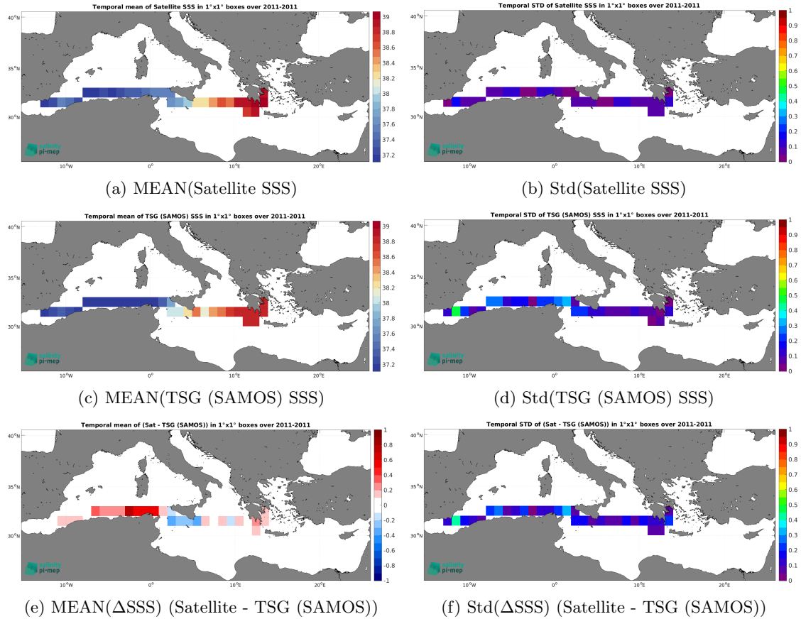
Figure 7: Temporal mean (left) and Std (right) of SSS from SMAP SSS L4 OI v3 - Daily (ESR) (top), TSG (SAMOS) (middle), and of \Delta\text{SSS} (Satellite - TSG (SAMOS)). Only match-up pairs are used to generate these maps.
