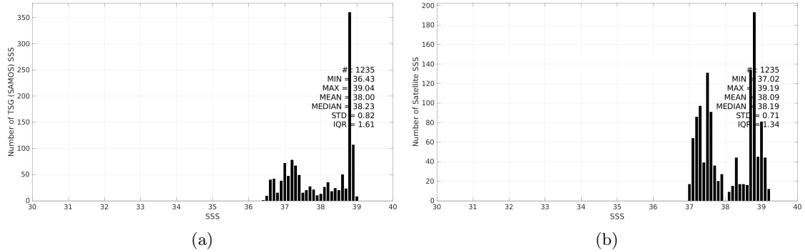
Figure 3: Histograms of SSS from TSG (SAMOS) (a) and SMAP SSS L4 OI v3 - Daily (ESR) (b) considering all match-up pairs per bins of 0.1 over the Mediterranean Sea Pi-MEP region and for the full satellite product period.
