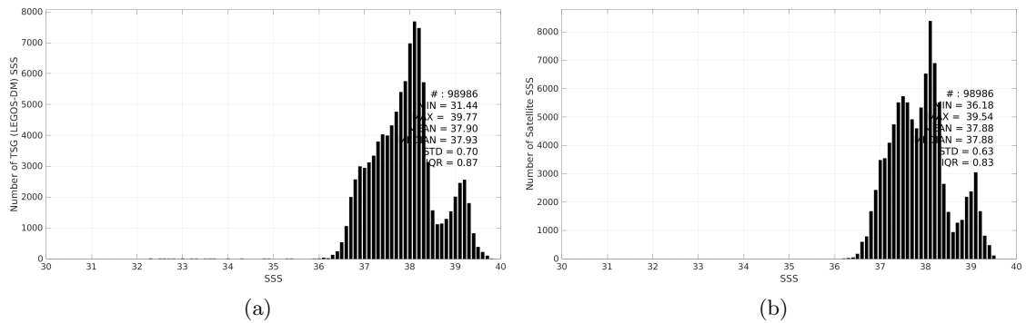
Figure 3: Histograms of SSS from TSG (LEGOS-DM) (a) and SMAP SSS L4 OI v3 - Daily (ESR) (b) considering all match-up pairs per bins of 0.1 over the Mediterranean Sea Pi-MEP region and for the full satellite product period.
