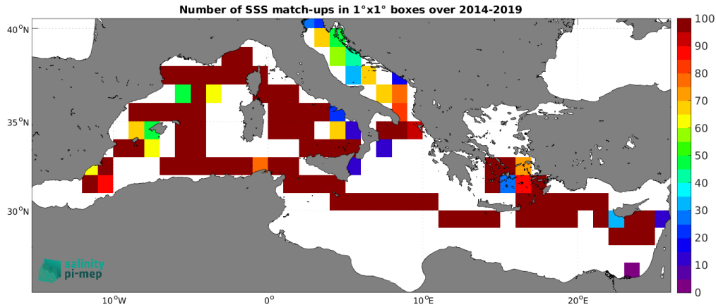
Figure 5: Number of SSS match-ups between TSG (GOSUD-Sailing-ship) SSS and the SMAP SSS L4 OI v3 - Daily (ESR) SSS product for the Mediterranean Sea Pi-MEP region over 1^\circ \times 1^\circ boxes and for the full satellite product period.
