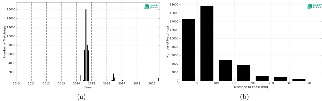
Figure 2: Number of match-ups between TSG (GOSUD-Sailing-ship) and SMAP SSS L4 OI v3 - Daily (ESR) SSS as a function of time (a) and as function of the distance to coast (b) over the Mediterranean Sea Pi-MEP region and for the full satellite product period.
