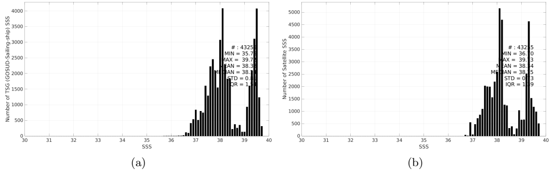
Figure 3: Histograms of SSS from TSG (GOSUD-Sailing-ship) (a) and SMAP SSS L4 OI v3 - Daily (ESR) (b) considering all match-up pairs per bins of 0.1 over the Mediterranean Sea Pi-MEP region and for the full satellite product period.
