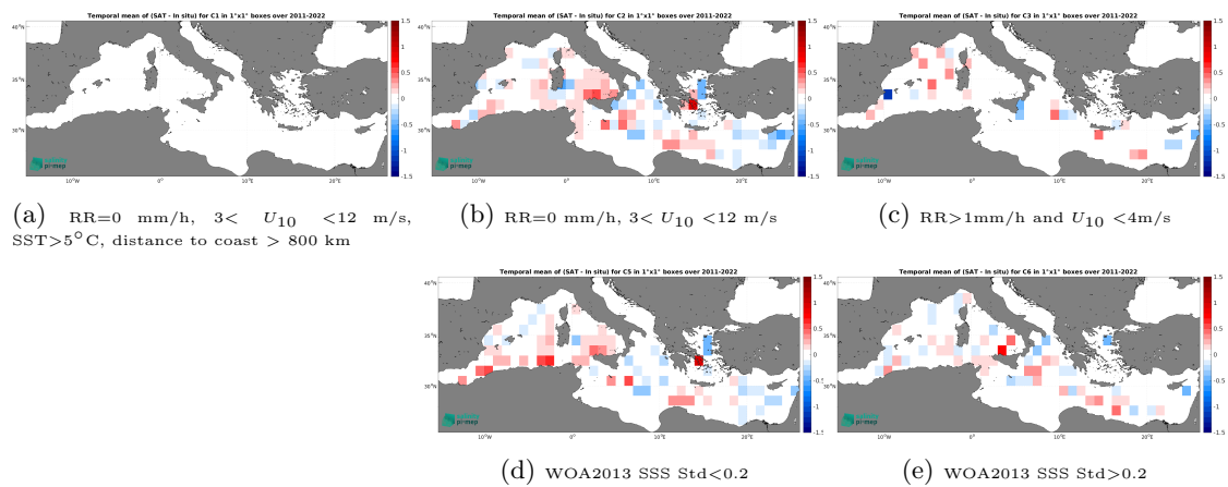
Figure 14: Temporal mean gridded over spatial boxes of size 1^\circ \times 1^\circ of \Delta\text{SSS} (SMAP SSS L4 OI v3 - Daily (ESR) - TSG (GOSUD-Research-vessel)) for 5 different subdatasets corresponding to:RR=0 mm/h, 3 < U_{10} < 12 m/s, SST>5°C, distance to coast > 800 km (a), RR=0 mm/h, 3 < U_{10} < 12 m/s (b), RR>1mm/h and U_{10} < 4 m/s (c), WOA2013 SSS Std<0.2 (d), WOA2013 SSS Std>0.2 (e).
