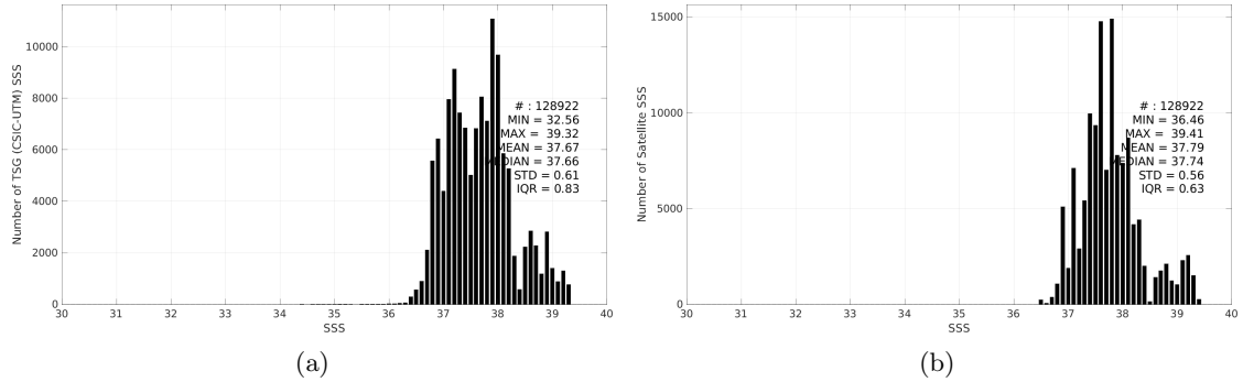
Figure 3: Histograms of SSS from TSG (CSIC-UTM) (a) and SMAP SSS L4 OI v3 - Daily (ESR) (b) considering all match-up pairs per bins of 0.1 over the Mediterranean Sea Pi-MEP region and for the full satellite product period.
