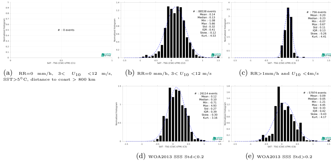
Figure 15: Normalized histogram of \Delta SSS (SMAP SSS L4 OI v3 - Daily (ESR) - TSG (CSIC-UTM)) for 5 different subdatasets corresponding to: RR=0 mm/h, 3 < U_{10} < 12 m/s, SST > 5°C, distance to coast > 800 km (a), RR=0 mm/h, 3 < U_{10} < 12 m/s (b), RR > 1mm/h and U_{10} < 4 m/s (c), WOA2013 SSS Std < 0.2 (d), WOA2013 SSS Std > 0.2 (e).
