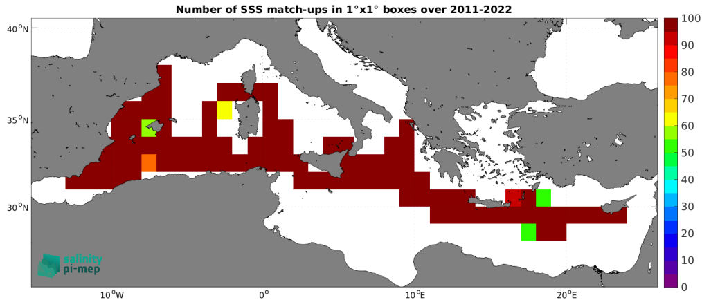
Figure 5: Number of SSS match-ups between TSG (CSIC-UTM) SSS and the SMAP SSS L4 OI v3 - Daily (ESR) SSS product for the Mediterranean Sea Pi-MEP region over 1^\circ \times 1^\circ boxes and for the full satellite product period.
