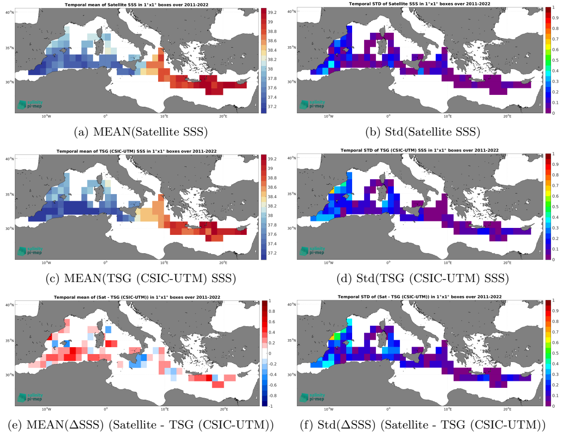
Figure 7: Temporal mean (left) and Std (right) of SSS from SMAP SSS L4 OI v3 - Daily (ESR) (top), TSG (CSIC-UTM) (middle), and of \Delta\text{SSS} (Satellite - TSG (CSIC-UTM)). Only match-up pairs are used to generate these maps.
