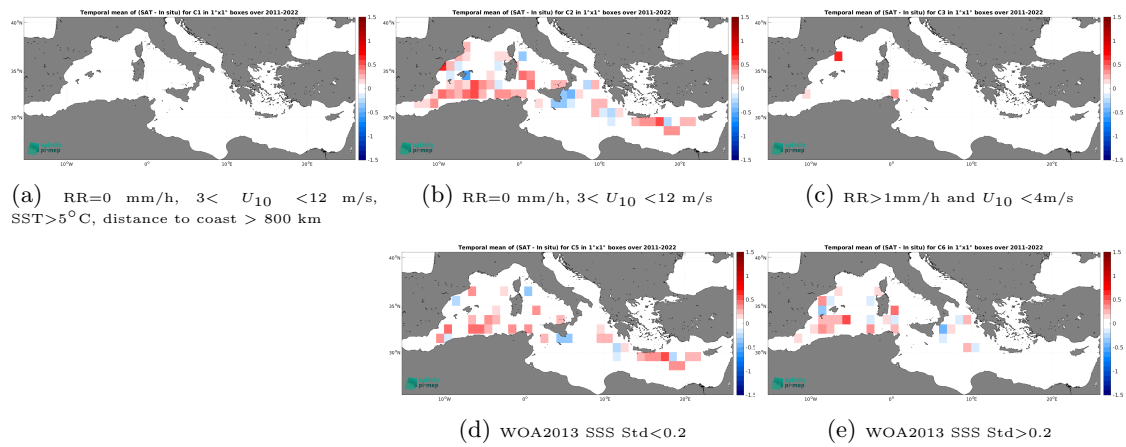
Figure 14: Temporal mean gridded over spatial boxes of size 1^\circ \times 1^\circ of \Delta SSS (SMAP SSS L4 OI v3 - Daily (ESR) - TSG (CSIC-UTM)) for 5 different subdatasets corresponding to:RR=0 mm/h, 3 < U_{10} < 12 m/s, SST>5°C, distance to coast > 800 km (a), RR=0 mm/h, 3 < U_{10} < 12 m/s (b), RR>1mm/h and U_{10} < 4 m/s (c), WOA2013 SSS Std<0.2 (d), WOA2013 SSS Std>0.2 (e).
