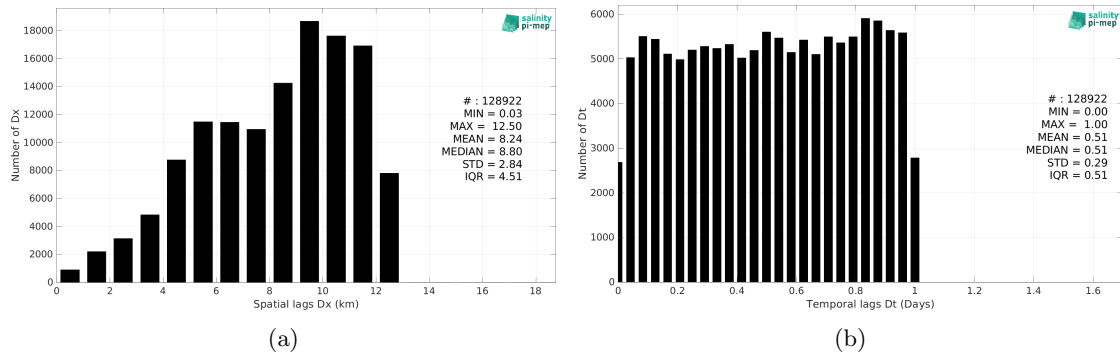
Figure 6: Histograms of the spatial (a) and temporal (b) lags between the location/time of the TSG (CSIC-UTM) measurement and the date of the corresponding SMAP SSS L4 OI v3 - Daily (ESR) SSS pixel.
