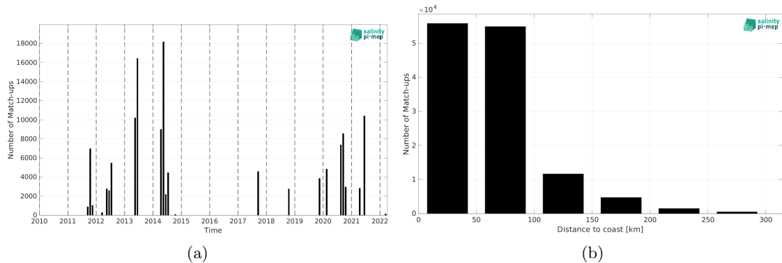
Figure 2: Number of match-ups between TSG (CSIC-UTM) and SMAP SSS L4 OI v3 - Daily (ESR) SSS as a function of time (a) and as function of the distance to coast (b) over the Mediterranean Sea Pi-MEP region and for the full satellite product period.
