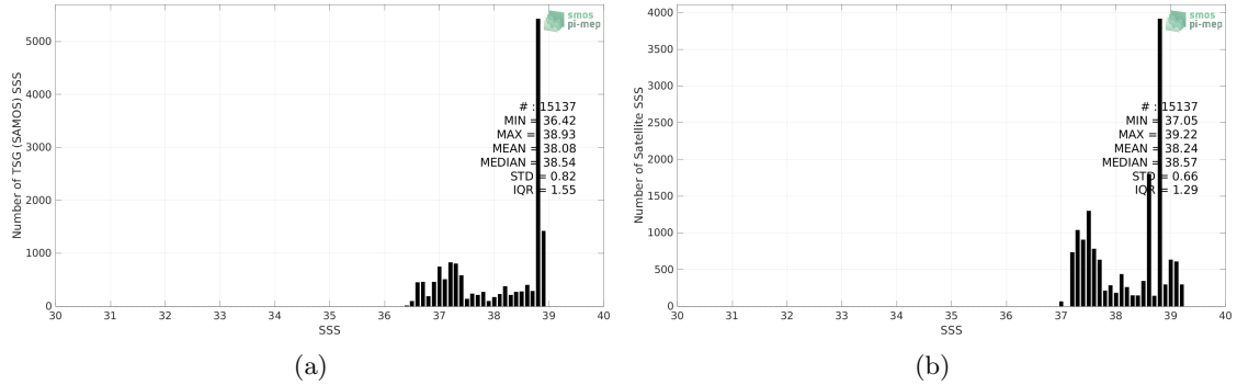
Figure 2: Histograms of SSS from TSG (SAMOS) (a) and SMAP SSS L4 OI v2 - 7 Days (ESR) (b) considering all match-up pairs per bins of 0.1 over the Mediterranean Sea Pi-MEP region and for the full satellite product period.
