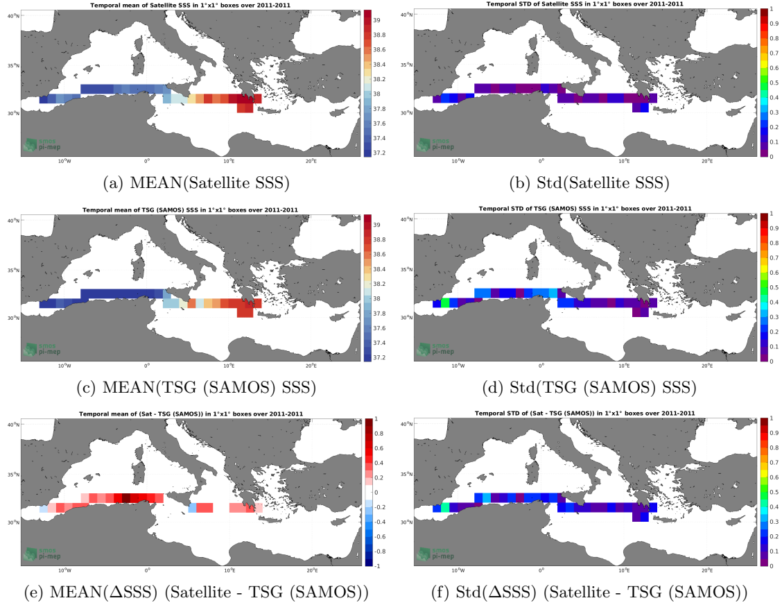
Figure 6: Temporal mean (left) and Std (right) of SSS from SMAP SSS L4 OI v2 - 7 Days (ESR) (top), TSG (SAMOS) (middle), and of \Delta\text{SSS} (Satellite - TSG (SAMOS)). Only match-up pairs are used to generate these maps.
