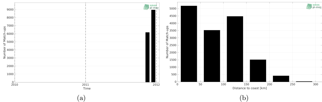
Figure 1: Number of match-ups between TSG (SAMOS) and SMAP SSS L4 OI v2 - 7 Days (ESR) SSS as a function of time (a) and as function of the distance to coast (b) over the Mediterranean Sea Pi-MEP region and for the full satellite product period.
