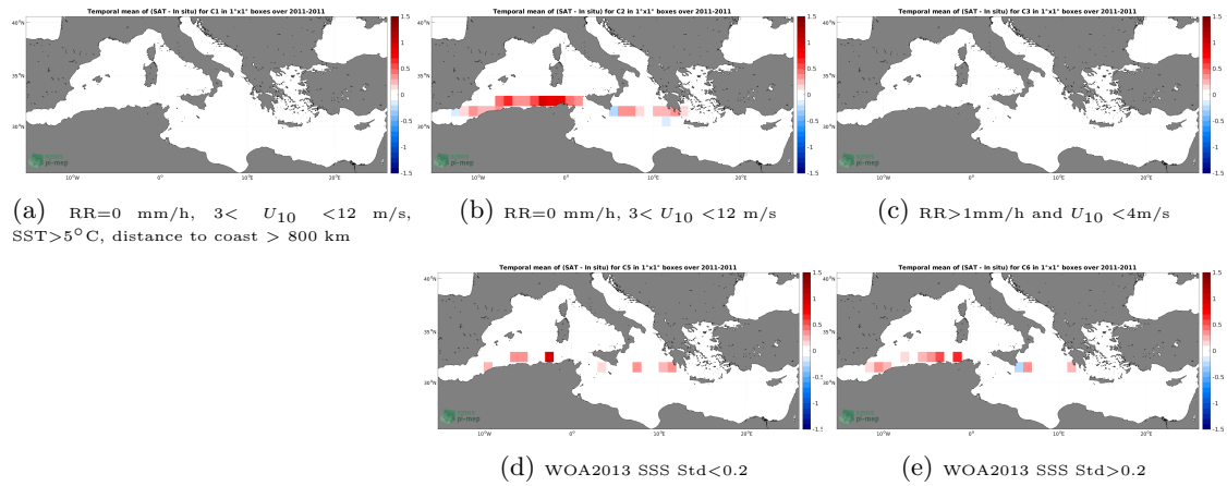
Figure 12: Temporal mean gridded over spatial boxes of size 1^{\circ}\times 1^{\circ} of \Delta\text{SSS} (SMAP SSS L4 OI v2 - 7 Days (ESR) - TSG (SAMOS)) for 5 different subdatasets corresponding to:RR=0 mm/h, 3 < U_{10} < 12 m/s, SST > 5^{\circ}\text{C} , distance to coast > 800 km (a), RR=0 mm/h, 3 < U_{10} < 12 m/s (b), RR > 1 mm/h and U_{10} < 4 m/s (c), WOA2013 SSS Std < 0.2 (d), WOA2013 SSS Std > 0.2 (e).
