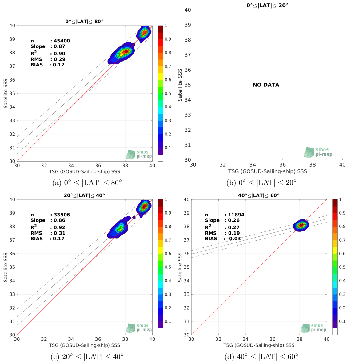
Figure 9: Contour maps of the concentration of SMAP SSS L4 OI v2 - 7 Days (ESR) SSS (y-axis) versus TSG (GOSUD-Sailing-ship) SSS (x-axis) at match-up pairs for different latitude bands. For each plot, the red line shows x=y . The black thin and dashed lines indicate a linear fit through the data cloud and the \pm 95\% confidence levels, respectively. The number match-up pairs n , the slope and R^2 coefficient of the linear fit, the root mean square (RMS) and the mean bias between satellite and in situ data are indicated for each latitude band in each plots.
