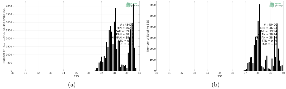
Figure 2: Histograms of SSS from TSG (GOSUD-Sailing-ship) (a) and SMAP SSS L4 OI v2 - 7 Days (ESR) (b) considering all match-up pairs per bins of 0.1 over the Mediterranean Sea Pi-MEP region and for the full satellite product period.
