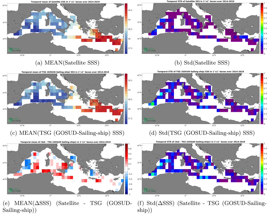
Figure 6: Temporal mean (left) and Std (right) of SSS from SMAP SSS L4 OI v2 - 7 Days (ESR) (top), TSG (GOSUD-Sailing-ship) (middle), and of \Delta\text{SSS} (Satellite - TSG (GOSUD-Sailing-ship)). Only match-up pairs are used to generate these maps.
