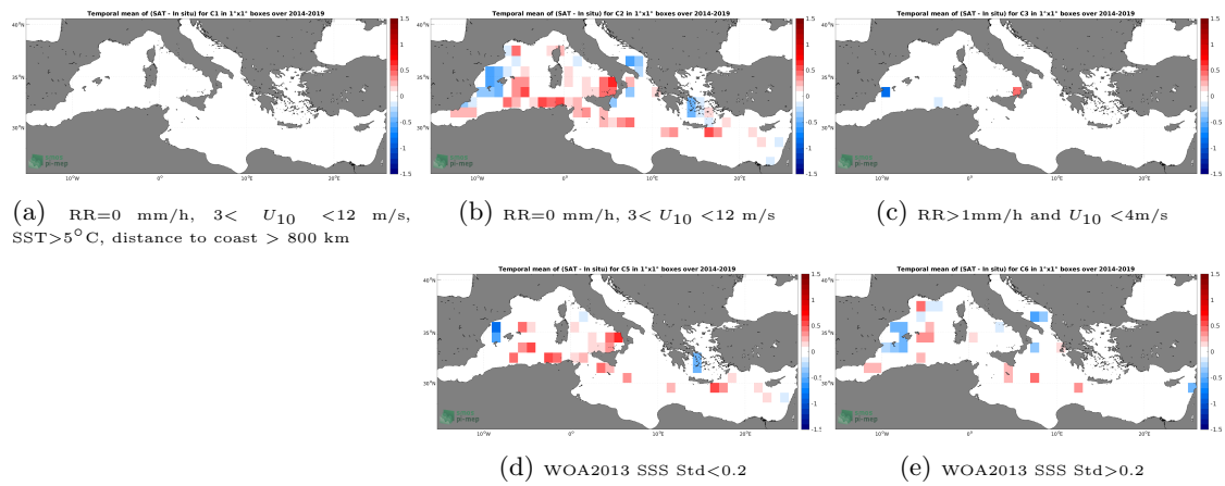
Figure 12: Temporal mean gridded over spatial boxes of size 1^\circ \times 1^\circ of \Delta SSS (SMAP SSS L4 OI v2 - 7 Days (ESR) - TSG (GOSUD-Sailing-ship)) for 5 different subdatasets corresponding to:RR=0 mm/h, 3 < U_{10} < 12 m/s, SST>5°C, distance to coast > 800 km (a), RR=0 mm/h, 3 < U_{10} < 12 m/s (b), RR>1mm/h and U_{10} < 4 m/s (c), WOA2013 SSS Std<0.2 (d), WOA2013 SSS Std>0.2 (e).
