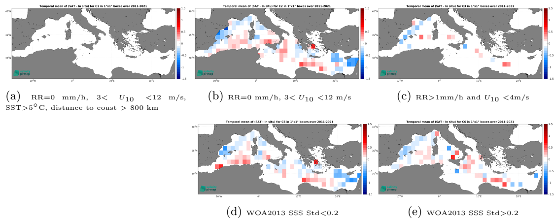
Figure 12: Temporal mean gridded over spatial boxes of size 1^\circ \times 1^\circ of \Delta\text{SSS} (SMAP SSS L4 OI v2 - 7 Days (ESR) - TSG (GOSUD-Research-vessel)) for 5 different subdatasets corresponding to:RR=0 mm/h, 3 < U_{10} < 12 m/s, SST>5°C, distance to coast > 800 km (a), RR=0 mm/h, 3 < U_{10} < 12 m/s (b), RR>1mm/h and U_{10} < 4 m/s (c), WOA2013 SSS Std<0.2 (d), WOA2013 SSS Std>0.2 (e).
