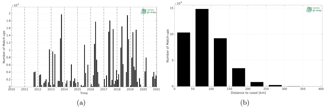
Figure 1: Number of match-ups between TSG (GOSUD-Research-vessel) and SMAP SSS L4 OI v2 - 7 Days (ESR) SSS as a function of time (a) and as function of the distance to coast (b) over the Mediterranean Sea Pi-MEP region and for the full satellite product period.
