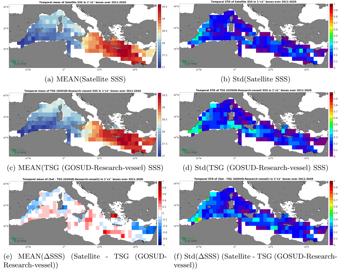
Figure 6: Temporal mean (left) and Std (right) of SSS from SMAP SSS L4 OI v2 - 7 Days (ESR) (top), TSG (GOSUD-Research-vessel) (middle), and of \Delta\text{SSS} (Satellite - TSG (GOSUD-Research-vessel)). Only match-up pairs are used to generate these maps.
