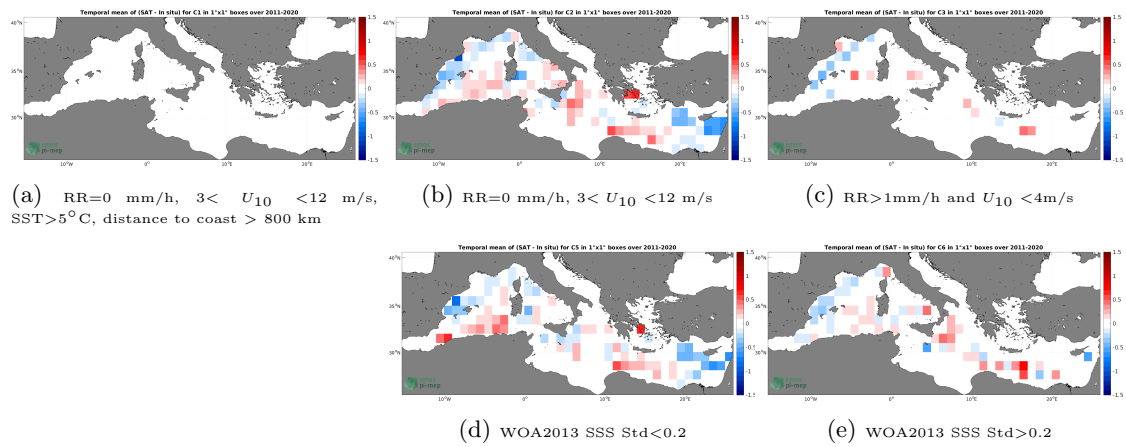
Figure 12: Temporal mean gridded over spatial boxes of size 1^\circ \times 1^\circ of \Delta SSS (SMAP SSS L4 OI v2 - 7 Days (ESR) - TSG (GOSUD-Research-vessel)) for 5 different subdatasets corresponding to:RR=0 mm/h, 3 < U_{10} < 12 m/s, SST>5°C, distance to coast > 800 km (a), RR=0 mm/h, 3 < U_{10} < 12 m/s (b), RR>1mm/h and U_{10} < 4 m/s (c), WOA2013 SSS Std<0.2 (d), WOA2013 SSS Std>0.2 (e).
