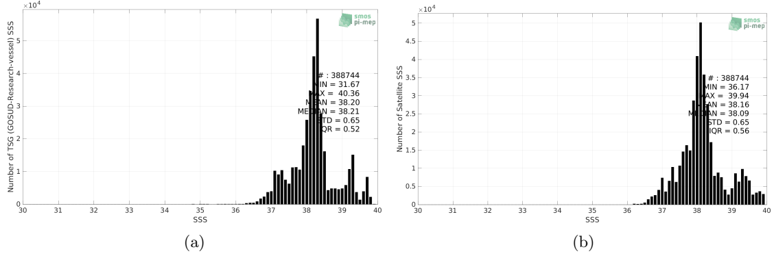
Figure 2: Histograms of SSS from TSG (GOSUD-Research-vessel) (a) and SMAP SSS L4 OI v2 - 7 Days (ESR) (b) considering all match-up pairs per bins of 0.1 over the Mediterranean Sea Pi-MEP region and for the full satellite product period.
