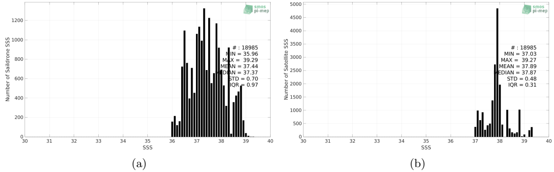
Figure 2: Histograms of SSS from Saildrone (a) and SMAP SSS L4 OI v2 - 7 Days (ESR) (b) considering all match-up pairs per bins of 0.1 over the Mediterranean Sea Pi-MEP region and for the full satellite product period.
