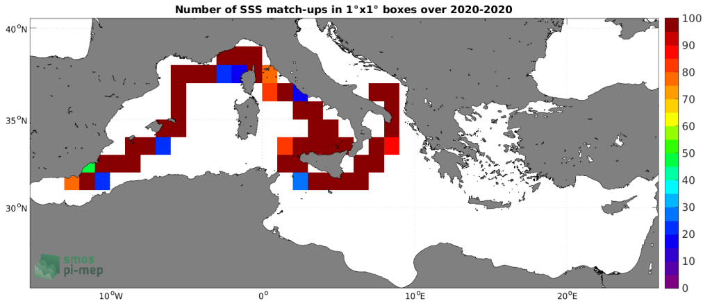
Figure 4: Number of SSS match-ups between Saildrone SSS and the SMAP SSS L4 OI v2 - 7 Days (ESR) SSS product for the Mediterranean Sea Pi-MEP region over 1^\circ \times 1^\circ boxes and for the full satellite product period.
