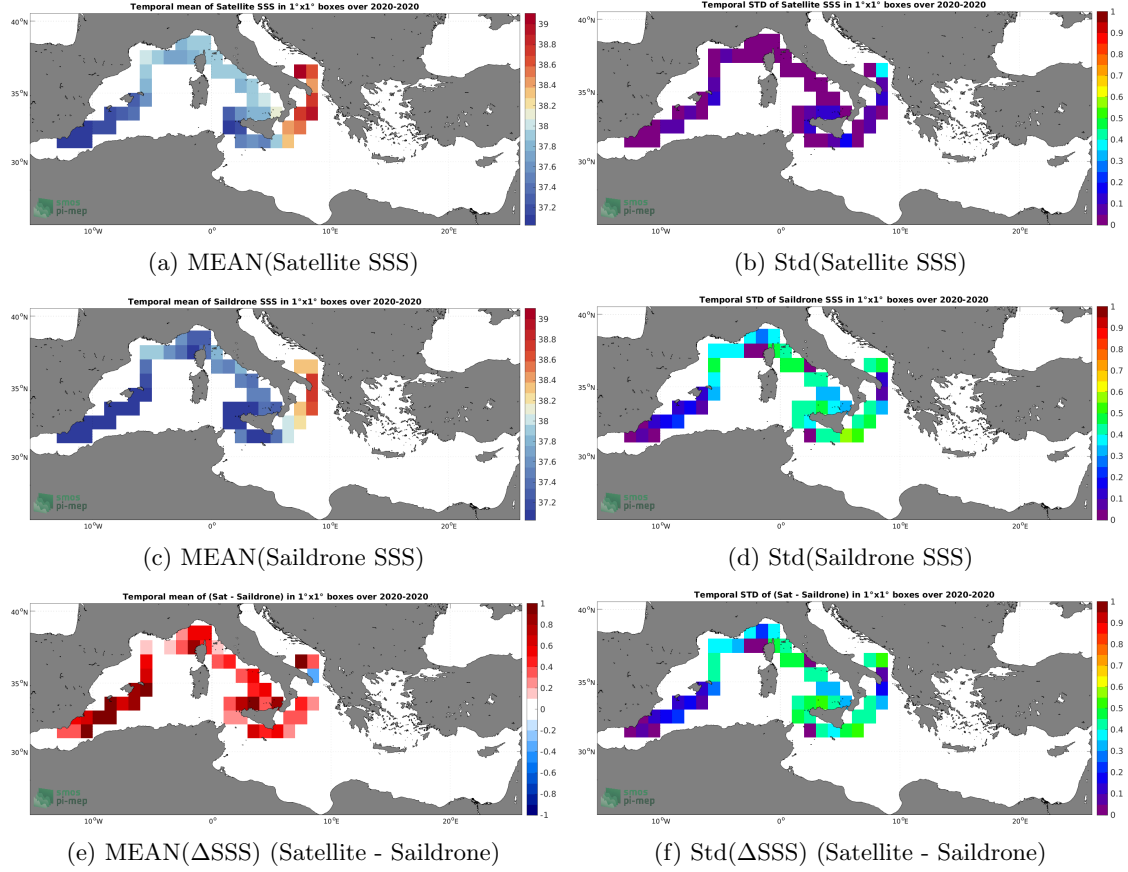
Figure 6: Temporal mean (left) and Std (right) of SSS from SMAP SSS L4 OI v2 - 7 Days (ESR) (top), Saildrone (middle), and of \Delta SSS (Satellite - Saildrone). Only match-up pairs are used to generate these maps.
