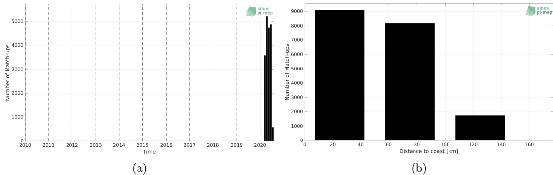
Figure 1: Number of match-ups between Saildrone and SMAP SSS L4 OI v2 - 7 Days (ESR) SSS as a function of time (a) and as function of the distance to coast (b) over the Mediterranean Sea Pi-MEP region and for the full satellite product period.
