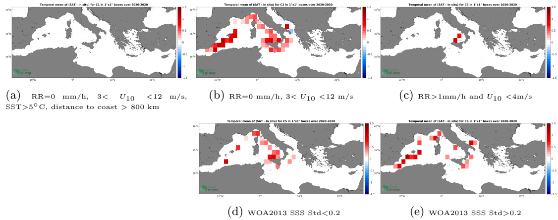
Figure 12: Temporal mean gridded over spatial boxes of size 1^\circ \times 1^\circ of \Delta SSS (SMAP SSS L4 OI v2 - 7 Days (ESR) - Saildrone) for 5 different subdatasets corresponding to:RR=0 mm/h, 3 < U_{10} < 12 m/s, SST >5^\circ\text{C} , distance to coast > 800 km (a), RR=0 mm/h, 3 < U_{10} < 12 m/s (b), RR >1 mm/h and U_{10} < 4 m/s (c), WOA2013 SSS Std <0.2 (d), WOA2013 SSS Std >0.2 (e).
