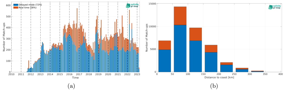
Figure 1: Number of match-ups between Argo and SMAP SSS L4 OI v2 - 7 Days (ESR) SSS as a function of time (a) and as function of the distance to coast (b) over the Mediterranean Sea Pi-MEP region and for the full satellite product period.
