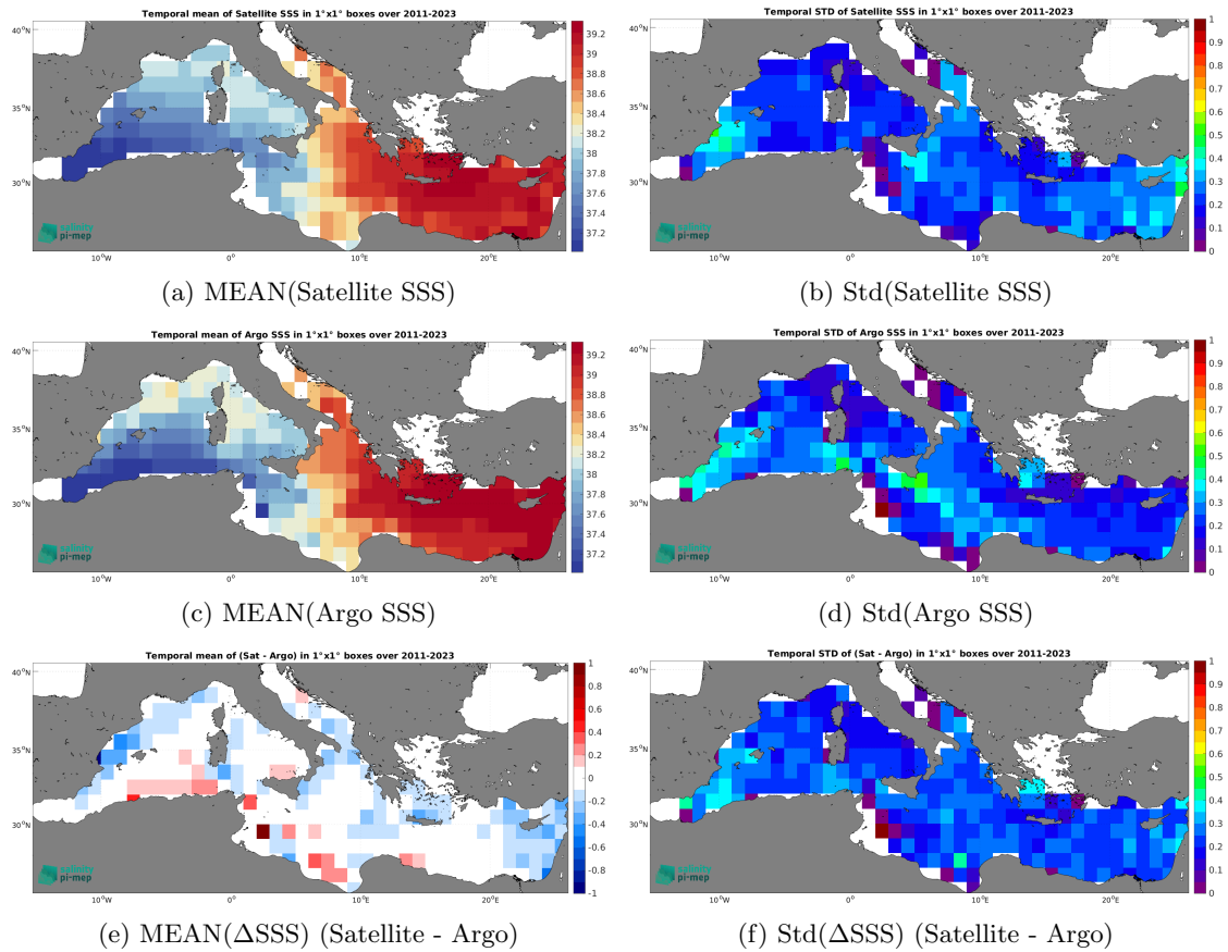
Figure 6: Temporal mean (left) and Std (right) of SSS from SMAP SSS L4 OI v2 - 7 Days (ESR) (top), Argo (middle), and of \Delta SSS (Satellite - Argo). Only match-up pairs are used to generate these maps.
