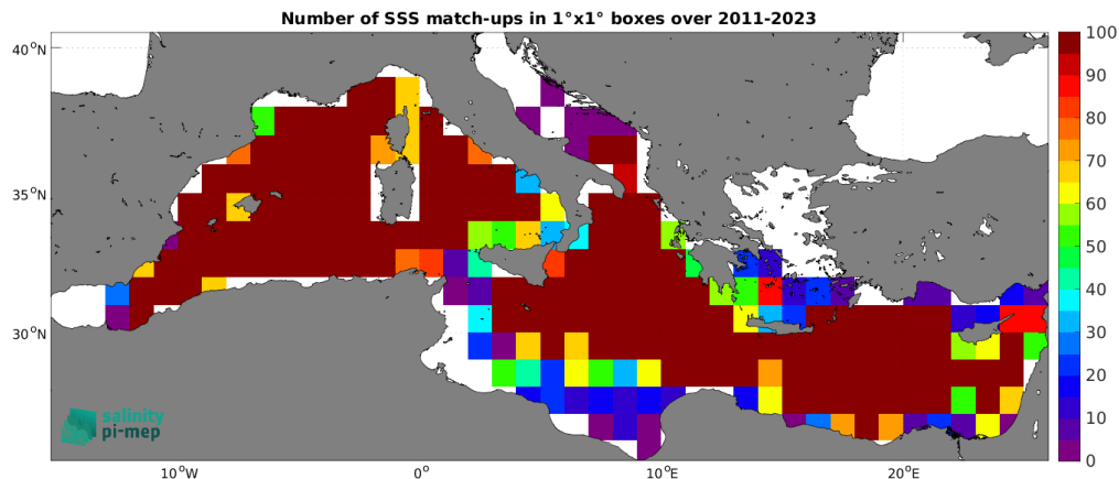
Figure 4: Number of SSS match-ups between Argo SSS and the SMAP SSS L4 OI v2 - 7 Days (ESR) SSS product for the Mediterranean Sea Pi-MEP region over 1^\circ \times 1^\circ boxes and for the full satellite product period.
