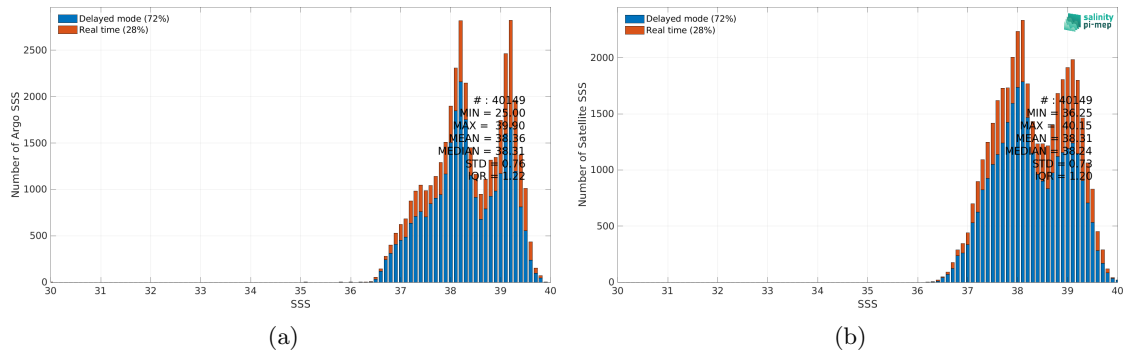
Figure 2: Histograms of SSS from Argo (a) and SMAP SSS L4 OI v2 - 7 Days (ESR) (b) considering all match-up pairs per bins of 0.1 over the Mediterranean Sea Pi-MEP region and for the full satellite product period.
