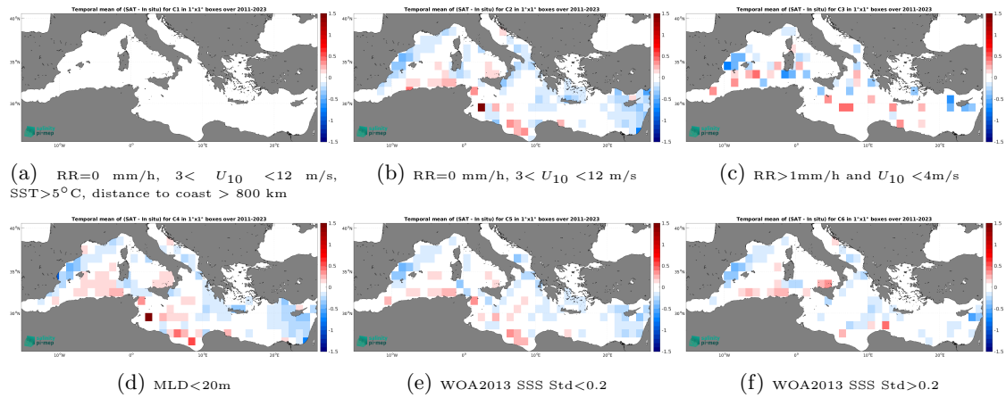
Figure 12: Temporal mean gridded over spatial boxes of size 1^\circ \times 1^\circ of \Delta SSS (SMAP SSS L4 OI v2 - 7 Days (ESR) - Argo) for 6 different subdatasets corresponding to:RR=0 mm/h, 3 < U_{10} < 12 m/s, SST >5^\circ C, distance to coast > 800 km (a), RR=0 mm/h, 3 < U_{10} < 12 m/s (b), RR >1 mm/h and U_{10} < 4 m/s (c),MLD <20 m (d),WOA2013 SSS Std <0.2 (e),WOA2013 SSS Std >0.2 (f).
