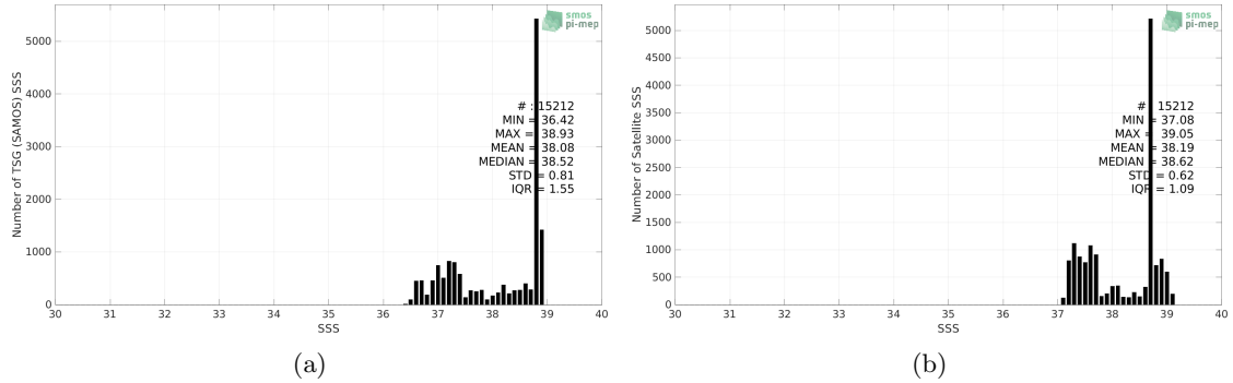
Figure 2: Histograms of SSS from TSG (SAMOS) (a) and SMAP SSS L4 OI v2 - Monthly (IPRC) (b) considering all match-up pairs per bins of 0.1 over the Mediterranean Sea Pi-MEP region and for the full satellite product period.
