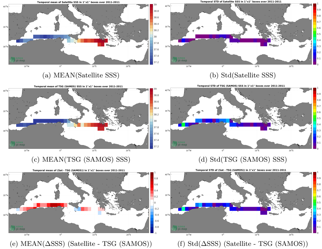
Figure 6: Temporal mean (left) and Std (right) of SSS from SMAP SSS L4 OI v2 - Monthly (IPRC) (top), TSG (SAMOS) ( in situ ) (middle), and of \Delta\text{SSS} (Satellite - TSG (SAMOS)). Only match-up pairs are used to generate these maps.
