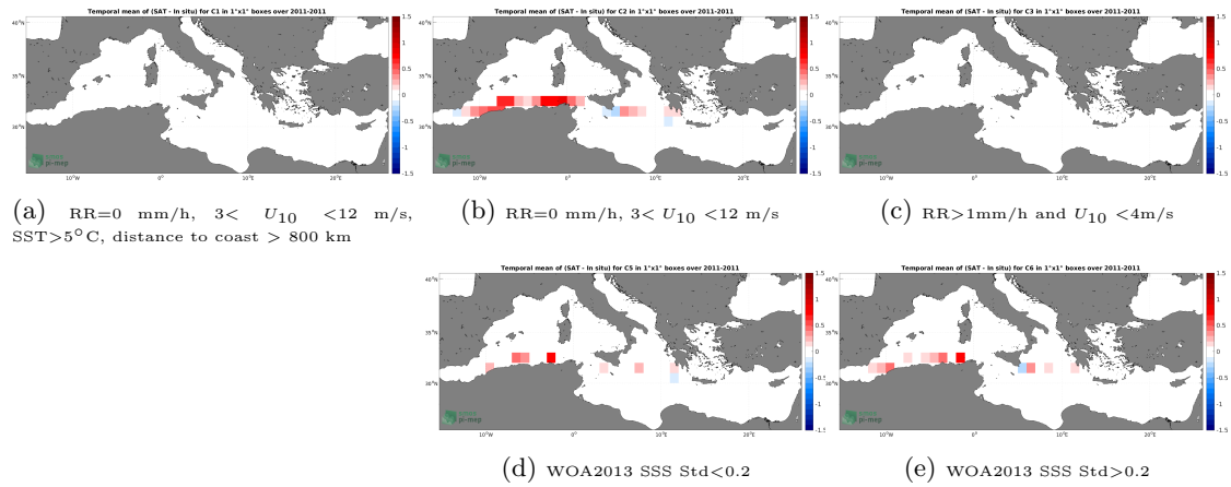
Figure 12: Temporal mean gridded over spatial boxes of size 1^{\circ}\times 1^{\circ} of \Delta\text{SSS} (SMAP SSS L4 OI v2 - Monthly (IPRC) - TSG (SAMOS)) for 5 different subdatasets corresponding to:RR=0 mm/h, 3 < U_{10} < 12 m/s, SST >5^{\circ}\text{C} , distance to coast > 800 km (a), RR=0 mm/h, 3 < U_{10} < 12 m/s (b), RR >1 mm/h and U_{10} < 4 m/s (c), WOA2013 SSS Std <0.2 (d), WOA2013 SSS Std >0.2 (e).
