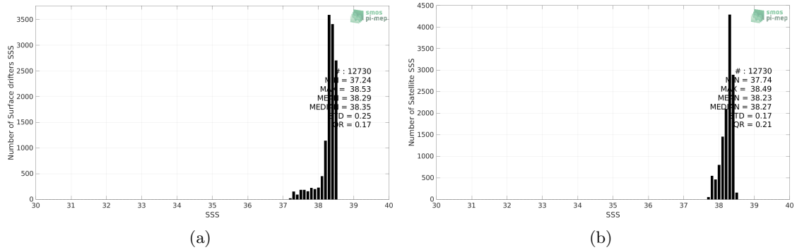
Figure 2: Histograms of SSS from Surface drifters (a) and SMAP SSS L4 OI v2 - Monthly (IPRC) (b) considering all match-up pairs per bins of 0.1 over the Mediterranean Sea Pi-MEP region and for the full satellite product period.
