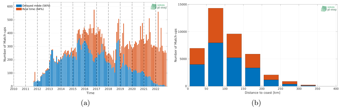
Figure 1: Number of match-ups between Argo and SMAP SSS L4 OI v2 - Monthly (IPRC) SSS as a function of time (a) and as function of the distance to coast (b) over the Mediterranean Sea Pi-MEP region and for the full satellite product period.
