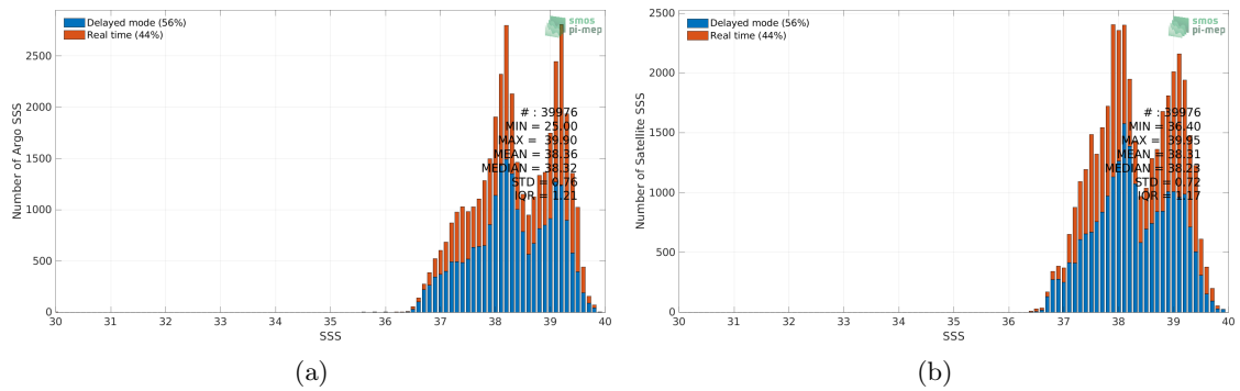
Figure 2: Histograms of SSS from Argo (a) and SMAP SSS L4 OI v2 - Monthly (IPRC) (b) considering all match-up pairs per bins of 0.1 over the Mediterranean Sea Pi-MEP region and for the full satellite product period.
