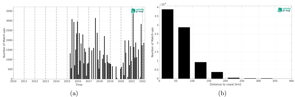
Figure 2: Number of match-ups between TSG (LEGOS-DM) and SMAP SSS L3 v6 - 8-Day running (RSS) SSS as a function of time (a) and as function of the distance to coast (b) over the Mediterranean Sea Pi-MEP region and for the full satellite product period.
