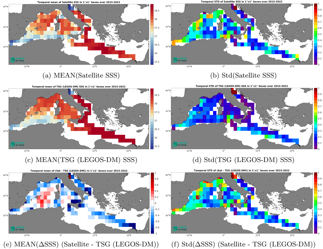
Figure 7: Temporal mean (left) and Std (right) of SSS from SMAP SSS L3 v6 - 8-Day running (RSS) (top), TSG (LEGOS-DM) (middle), and of \Delta\text{SSS} (Satellite - TSG (LEGOS-DM)). Only match-up pairs are used to generate these maps.
