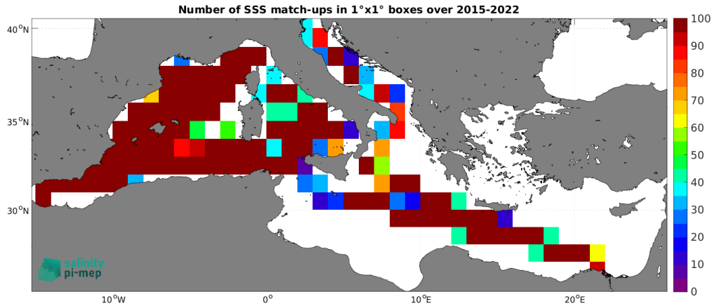
Figure 5: Number of SSS match-ups between TSG (LEGOS-DM) SSS and the SMAP SSS L3 v6 - 8-Day running (RSS) SSS product for the Mediterranean Sea Pi-MEP region over 1^\circ \times 1^\circ boxes and for the full satellite product period.
