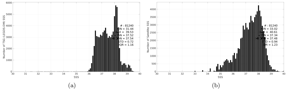
Figure 3: Histograms of SSS from TSG (LEGOS-DM) (a) and SMAP SSS L3 v6 - 8-Day running (RSS) (b) considering all match-up pairs per bins of 0.1 over the Mediterranean Sea Pi-MEP region and for the full satellite product period.
