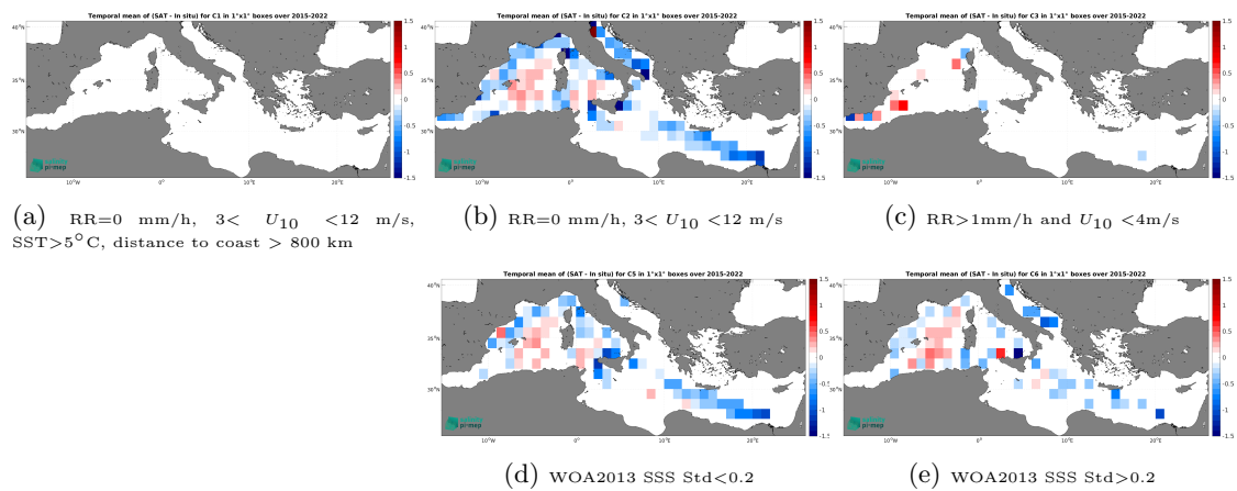
Figure 14: Temporal mean gridded over spatial boxes of size 1^\circ \times 1^\circ of \Delta\text{SSS} (SMAP SSS L3 v6 - 8-Day running (RSS) - TSG (LEGOS-DM)) for 5 different subdatasets corresponding to:RR=0 mm/h, 3 < U_{10} < 12 m/s, SST>5°C, distance to coast > 800 km (a), RR=0 mm/h, 3 < U_{10} < 12 m/s (b), RR>1mm/h and U_{10} < 4 m/s (c), WOA2013 SSS Std<0.2 (d), WOA2013 SSS Std>0.2 (e).
