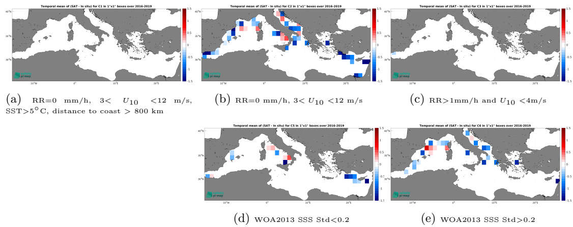
Figure 14: Temporal mean gridded over spatial boxes of size 1^\circ \times 1^\circ of \Delta\text{SSS} (SMAP SSS L3 v6 - 8-Day running (RSS) - TSG (GOSUD-Sailing-ship)) for 5 different subdatasets corresponding to:RR=0 mm/h, 3 < U_{10} < 12 m/s, SST >5^\circ\text{C} , distance to coast > 800 km (a), RR=0 mm/h, 3 < U_{10} < 12 m/s (b), RR >1 mm/h and U_{10} < 4 m/s (c), WOA2013 SSS Std <0.2 (d), WOA2013 SSS Std >0.2 (e).
