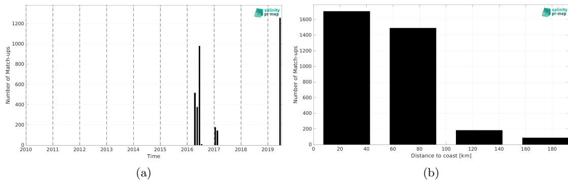
Figure 2: Number of match-ups between TSG (GOSUD-Sailing-ship) and SMAP SSS L3 v6 - 8-Day running (RSS) SSS as a function of time (a) and as function of the distance to coast (b) over the Mediterranean Sea Pi-MEP region and for the full satellite product period.
