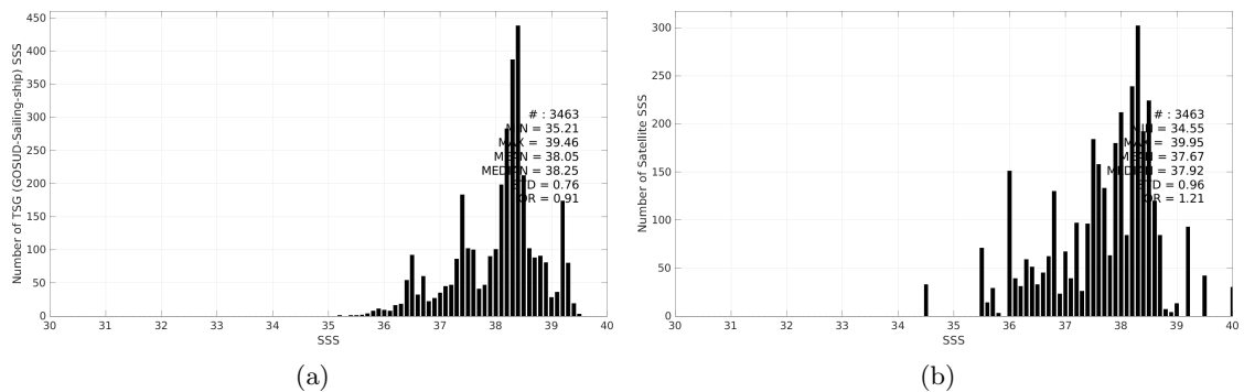
Figure 3: Histograms of SSS from TSG (GOSUD-Sailing-ship) (a) and SMAP SSS L3 v6 - 8-Day running (RSS) (b) considering all match-up pairs per bins of 0.1 over the Mediterranean Sea Pi-MEP region and for the full satellite product period.
