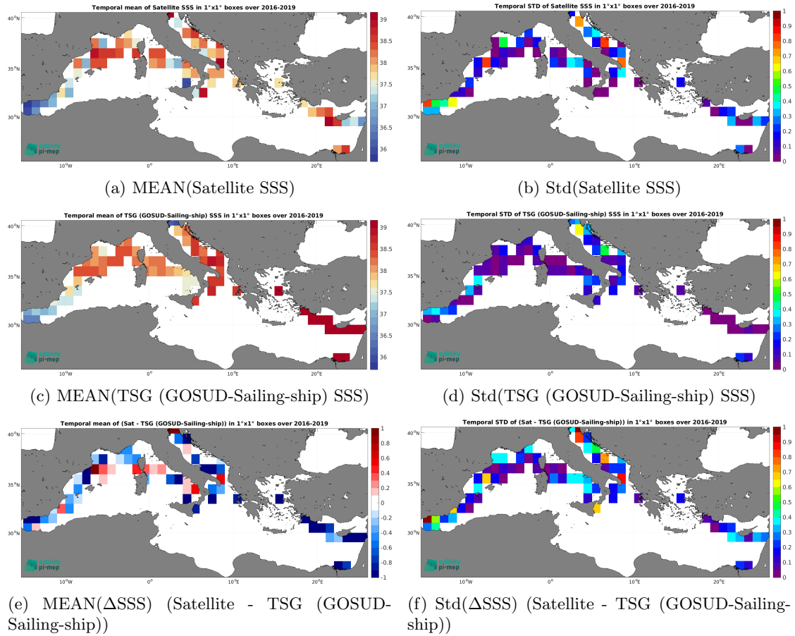
Figure 7: Temporal mean (left) and Std (right) of SSS from SMAP SSS L3 v6 - 8-Day running (RSS) (top), TSG (GOSUD-Sailing-ship) (middle), and of \Delta SSS (Satellite - TSG (GOSUD-Sailing-ship)). Only match-up pairs are used to generate these maps.
