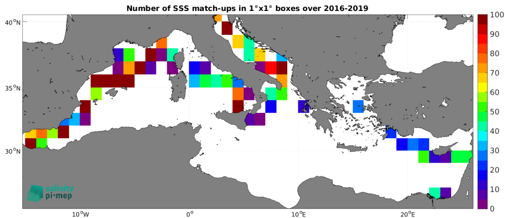
Figure 5: Number of SSS match-ups between TSG (GOSUD-Sailing-ship) SSS and the SMAP SSS L3 v6 - 8-Day running (RSS) SSS product for the Mediterranean Sea Pi-MEP region over 1^\circ \times 1^\circ boxes and for the full satellite product period.
