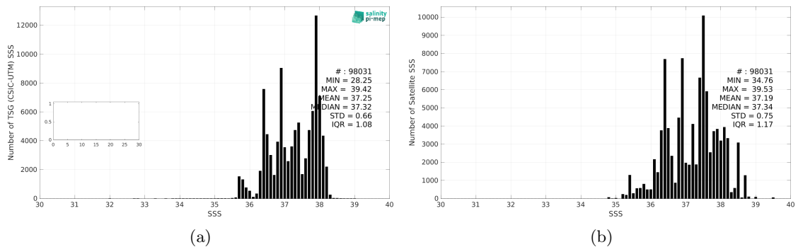
Figure 3: Histograms of SSS from TSG (CSIC-UTM) (a) and SMAP SSS L3 v6 - 8-Day running (RSS) (b) considering all match-up pairs per bins of 0.1 over the Mediterranean Sea Pi-MEP region and for the full satellite product period.
