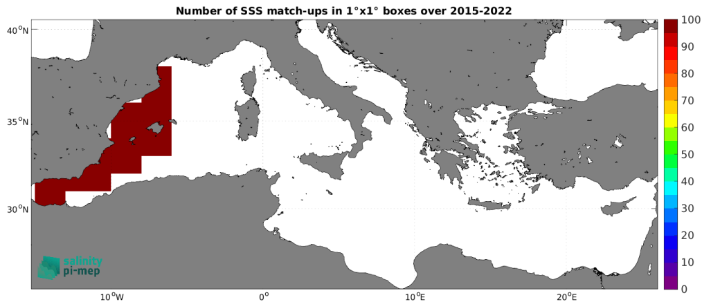
Figure 5: Number of SSS match-ups between TSG (CSIC-UTM) SSS and the SMAP SSS L3 v6 - 8-Day running (RSS) SSS product for the Mediterranean Sea Pi-MEP region over 1^\circ \times 1^\circ boxes and for the full satellite product period.
