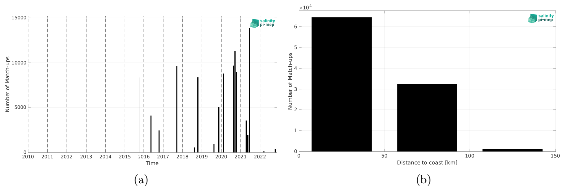
Figure 2: Number of match-ups between TSG (CSIC-UTM) and SMAP SSS L3 v6 - 8-Day running (RSS) SSS as a function of time (a) and as function of the distance to coast (b) over the Mediterranean Sea Pi-MEP region and for the full satellite product period.
