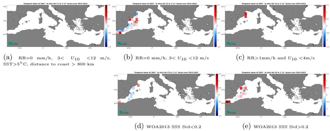
Figure 14: Temporal mean gridded over spatial boxes of size 1^\circ \times 1^\circ of \Delta\text{SSS} (SMAP SSS L3 v6 - 8-Day running (RSS) - TSG (CSIC-UTM)) for 5 different subdatasets corresponding to:RR=0 mm/h, 3 < U_{10} < 12 m/s, SST>5°C, distance to coast > 800 km (a), RR=0 mm/h, 3 < U_{10} < 12 m/s (b), RR>1mm/h and U_{10} < 4 m/s (c), WOA2013 SSS Std<0.2 (d), WOA2013 SSS Std>0.2 (e).
