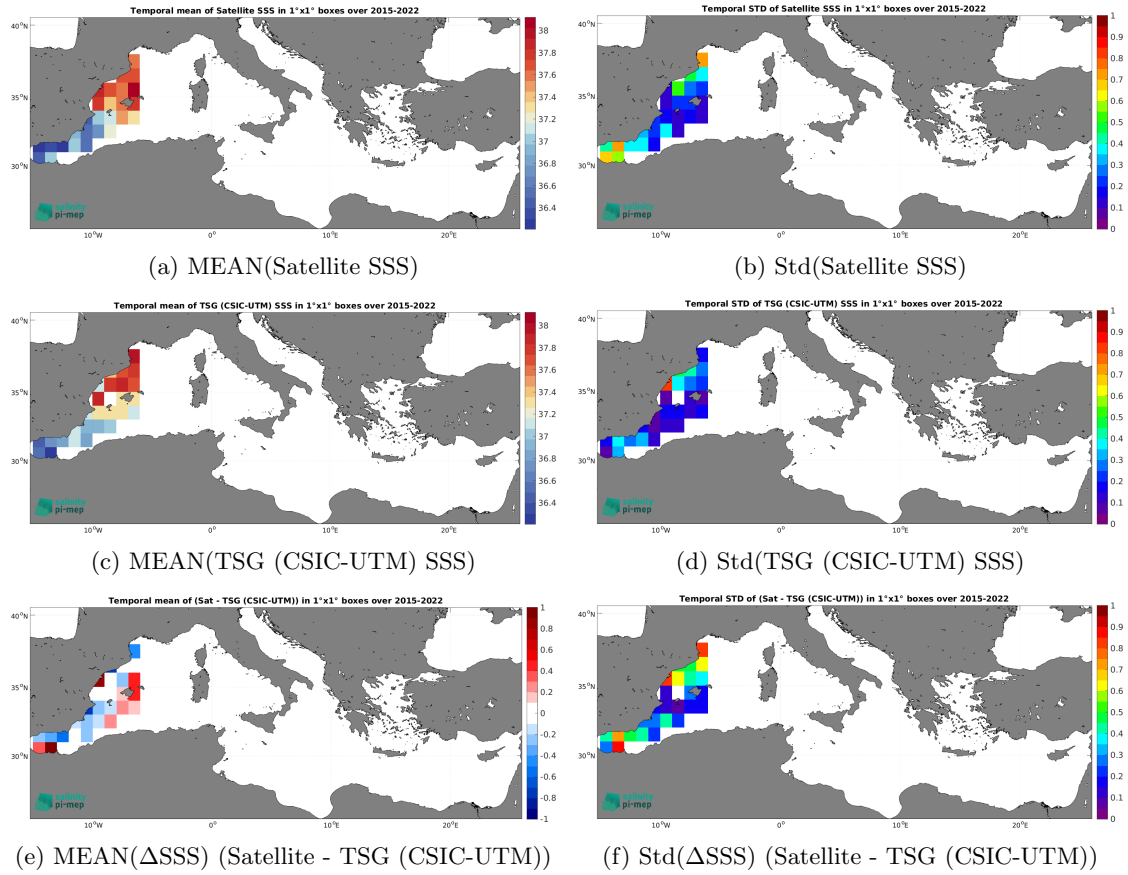
Figure 7: Temporal mean (left) and Std (right) of SSS from SMAP SSS L3 v6 - 8-Day running (RSS) (top), TSG (CSIC-UTM) (middle), and of \Delta SSS (Satellite - TSG (CSIC-UTM)). Only match-up pairs are used to generate these maps.
