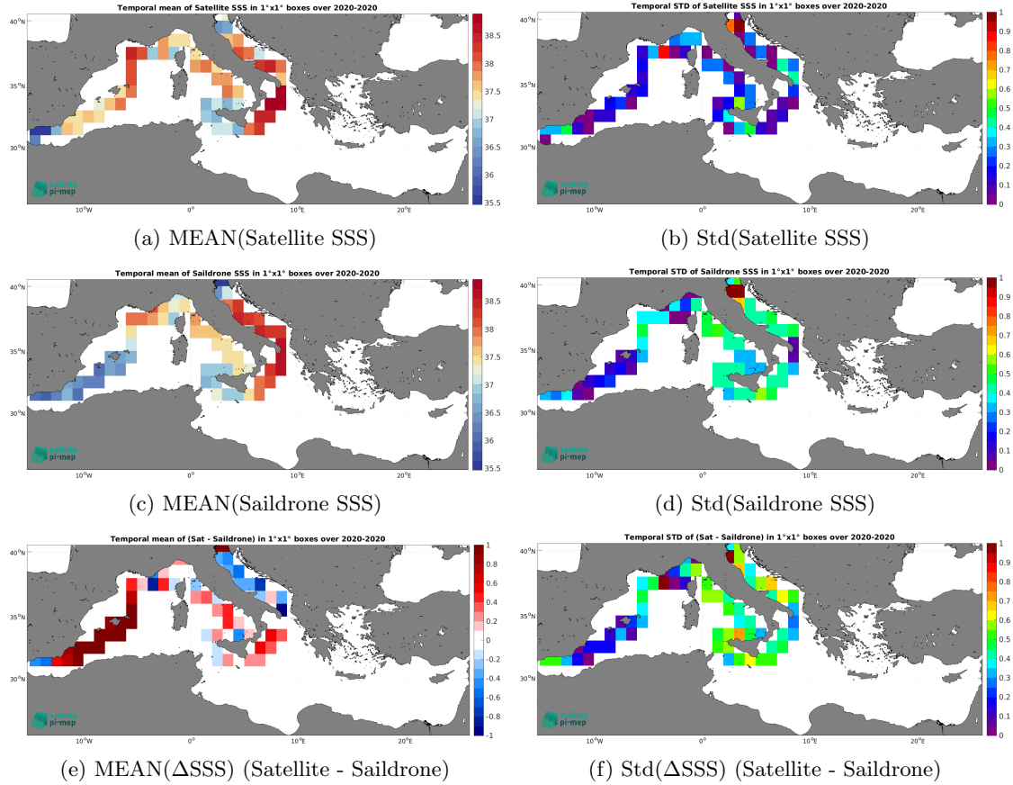
Figure 7: Temporal mean (left) and Std (right) of SSS from SMAP SSS L3 v6 - 8-Day running (RSS) (top), Saildrone (middle), and of \Delta SSS (Satellite - Saildrone). Only match-up pairs are used to generate these maps.
