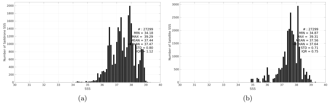
Figure 3: Histograms of SSS from Saildrone (a) and SMAP SSS L3 v6 - 8-Day running (RSS) (b) considering all match-up pairs per bins of 0.1 over the Mediterranean Sea Pi-MEP region and for the full satellite product period.
