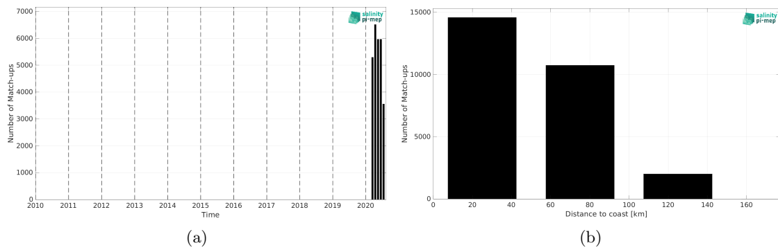
Figure 2: Number of match-ups between Saildrone and SMAP SSS L3 v6 - 8-Day running (RSS) SSS as a function of time (a) and as function of the distance to coast (b) over the Mediterranean Sea Pi-MEP region and for the full satellite product period.
