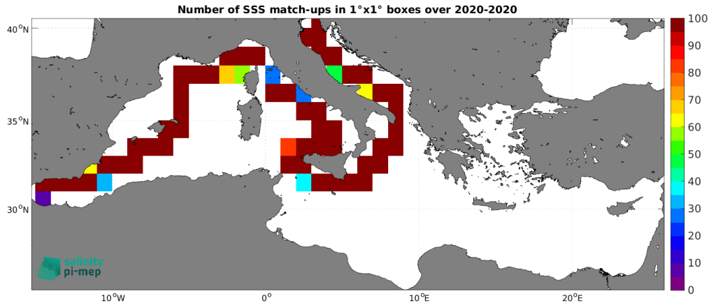
Figure 5: Number of SSS match-ups between Saildrone SSS and the SMAP SSS L3 v6 - 8-Day running (RSS) SSS product for the Mediterranean Sea Pi-MEP region over 1^\circ \times 1^\circ boxes and for the full satellite product period.
