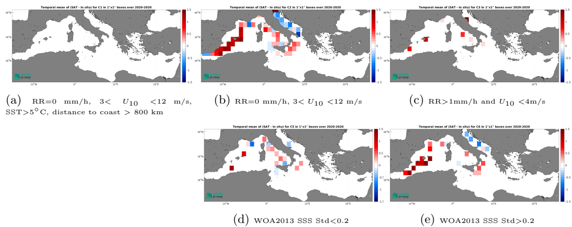
Figure 14: Temporal mean gridded over spatial boxes of size 1^\circ \times 1^\circ of \Delta SSS (SMAP SSS L3 v6 - 8-Day running (RSS) - Saildrone) for 5 different subdatasets corresponding to:RR=0 mm/h, 3 < U_{10} < 12 m/s, SST >5^\circ\text{C} , distance to coast > 800 km (a), RR=0 mm/h, 3 < U_{10} < 12 m/s (b), RR >1 mm/h and U_{10} < 4 m/s (c), WOA2013 SSS Std <0.2 (d), WOA2013 SSS Std >0.2 (e).
