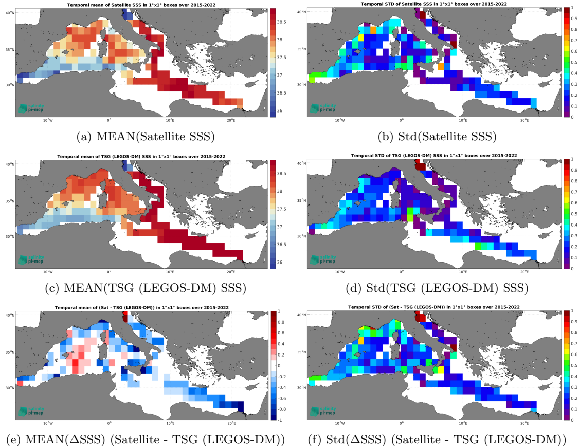
Figure 7: Temporal mean (left) and Std (right) of SSS from SMAP SSS L3 v6 - Monthly (RSS) (top), TSG (LEGOS-DM) (middle), and of \Delta\text{SSS} (Satellite - TSG (LEGOS-DM)). Only match-up pairs are used to generate these maps.
