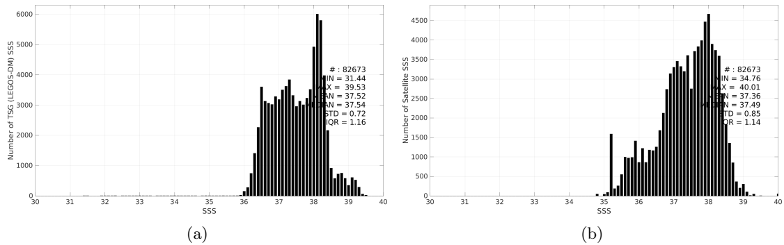
Figure 3: Histograms of SSS from TSG (LEGOS-DM) (a) and SMAP SSS L3 v6 - Monthly (RSS) (b) considering all match-up pairs per bins of 0.1 over the Mediterranean Sea Pi-MEP region and for the full satellite product period.
