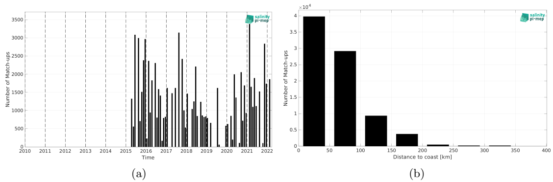
Figure 2: Number of match-ups between TSG (LEGOS-DM) and SMAP SSS L3 v6 - Monthly (RSS) SSS as a function of time (a) and as function of the distance to coast (b) over the Mediterranean Sea Pi-MEP region and for the full satellite product period.
