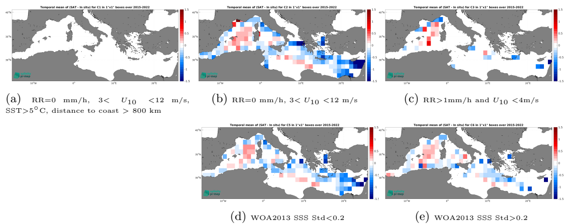
Figure 14: Temporal mean gridded over spatial boxes of size 1^\circ \times 1^\circ of \Delta\text{SSS} (SMAP SSS L3 v6 - Monthly (RSS) - TSG (GOSUD-Research-vessel)) for 5 different subdatasets corresponding to:RR=0 mm/h, 3 < U_{10} < 12 m/s, SST >5^\circ\text{C} , distance to coast > 800 km (a), RR=0 mm/h, 3 < U_{10} < 12 m/s (b), RR >1 mm/h and U_{10} < 4 m/s (c), WOA2013 SSS Std <0.2 (d), WOA2013 SSS Std >0.2 (e).
